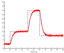
(a) p = 0.05 : output variable and reference trajectory
