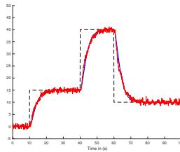
(c) p = 0.5 : output variable and reference trajectory
