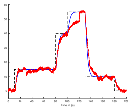
(g) Output variable and reference trajectory
