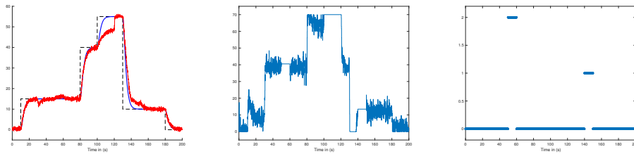
(a) Output variable and reference trajectory (b) Control variable (c) 0: no loss, 1: fault 1, 2: fault 2
