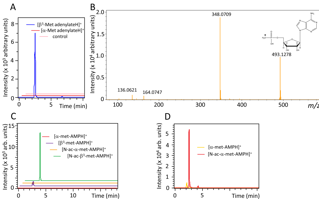
Fig. 4. LC-HRMS analyses of MGL-treated \beta^3 -Met activation and transfer onto tRNA^{\text{Met}} . Panel A: Analysis of the products of the activation reaction. The red and blue chromatograms in correspond to the sample in which MetRS was reacted with ATP and MGL-treated \beta^3 -Met. Extracted ion current (EIC) chromatograms of m/z 479.111 \pm 0.001 (red, corresponding to [\alpha\text{-Met adenylateH}]^+ C_{15}H_{24}N_6O_8PS ) and of m/z 493.126 \pm 0.001 (blue, corresponding to [\beta^3\text{-Met adenylateH}]^+ C_{16}H_{26}N_6O_8PS ). The pink chromatogram corresponds to m/z 493.126 \pm 0.001 ( [\beta^3\text{-Met adenylateH}]^+ ) for the zero reaction time control sample. Panel B: HR-MS/MS ( E_{\text{col}} = 15 eV) of the m/z 493.1263 ion obtained at 2.6 min retention time (blue chromatogram in Panel A). The proposed mechanism for the decomposition of the molecular ion is indicated on the Supplementary Scheme 1. Panel C: LC-HRMS analysis of the aminoacylation reaction in the presence of MGL-treated \beta^3 -Met. The samples were submitted to S1 nuclease cleavage as indicated in Materials and Methods. The panel shows the extracted ion current chromatograms (EIC) of m/z 479.111 \pm 0.001 (corresponding to [\alpha\text{-methionyl-AMPH}]^+ , C_{15}H_{24}N_6O_8PS ; red) and m/z 493.126 \pm 0.001 (corresponding to [\beta^3\text{-methionyl-AMPH}]^+ , C_{16}H_{26}N_6O_8PS ; purple). The two other chromatograms correspond to the samples acetylated prior to S1 cleavage, showing the EIC of m/z 521.121 \pm 0.001 (corresponding to [\text{N-acetyl-}\alpha\text{-methionyl-AMPH}]^+ , C_{17}H_{26}N_6O_9PS ; orange) and m/z 535.138 (corresponding to [\text{N-acetyl-}\beta^3\text{-methionyl-AMPH}]^+ , C_{18}H_{28}N_6O_9PS ; green). The panel shows the presence of the compounds expected from the transfer of \beta^3 -Met onto tRNA and the absence of detectable aminoacylation with \alpha -Met. Panel D: Reference aminoacylation experiment using \alpha -Met instead of \beta^3 -Met, with (red) or without (yellow) acetylation. The panel shows the EIC of m/z 479.111 \pm 0.001 (corresponding to [\alpha\text{-methionyl-AMPH}]^+ , C_{15}H_{24}N_6O_8PS ; yellow) and m/z 521.121 \pm 0.001 (corresponding to [\text{N-acetyl-}\alpha\text{-methionyl-AMPH}]^+ , C_{17}H_{26}N_6O_9PS ; red). The ions at m/z 535.138 ( [\text{N-acetyl-}\beta^3\text{-methionyl-AMPH}]^+ ) and m/z 521.121 ( [\text{N-acetyl-}\alpha\text{-methionyl-AMPH}]^+ ) were further characterized by HR-MS/MS (Supplementary Table 1 and Supplementary Scheme 2). (For interpretation of the references to colour in this figure legend, the reader is referred to the web version of this article.)
