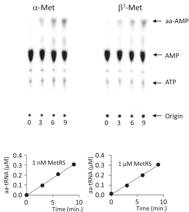
Fig. 5. Aminoacylation of tRNA_f^{Met} by MGL-treated \beta^3 -Met. [ 3' - ^{32}P ]-labelled tRNA_f^{Met} was aminoacylated with \alpha -Met in the presence of 1 nM MetRS or with MGL-treated \beta^3 -Met in the presence of 1 \mu M MetRS (see Materials and Methods). At the indicated times, aliquots were withdrawn and digested with S1 nuclease. The resulting digests were analyzed by TLC. The figure shows the results of a typical experiment with the fluorogram in the upper part and the corresponding image analysis in the bottom part. The figure shows that the rates differ by three orders of magnitude. The average rates from two independent experiments are reported in Table 1.
