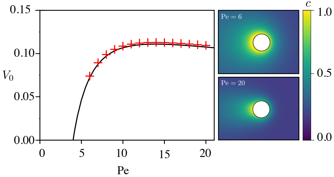
FIG. 3: Mean self-propulsion velocity V_0 of two active droplets with \bar{\eta} = 1/36 initially located at a distance d = 48 from each other (red crosses). The results of Ref. [17] for a single active droplet with the same viscosity ratio are also reported (black solid line), and the concentration distribution around the self-propelling droplets is shown for Pe = 6 and Pe = 20 .
