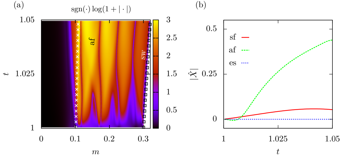
Figure 3: (a) Intensity map in the variables (m, t) of the local Euclidean norm of the solution to (4) with optimal initial condition for final time T = 1.05 and k_{\perp} = 0.1 . (b) Time evolution of the deformations of the external surface (blue), the ablation front (green) and the shock front (red).
