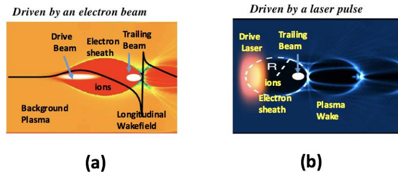
Fig.2 Nonlinear plasma wakes produced by a) an electron beam and b) a laser pulse. In both cases the drive pulses are travelling from the right to the left. In a) the black curve shows the on-axis longitudinal electric field of the wake.
