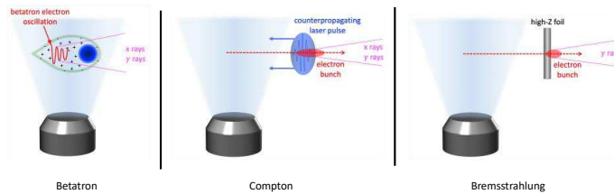
Figure 7 – Principle of betatron, inverse-Compton and bremsstrahlung radiation sources. In the first case (left), electrons oscillate in the blow-out cavity of the laser-plasma accelerator and radiate betatron x rays. For the inverse-Compton source (middle), at the exit of the laser-plasma accelerator, electrons radiates IC scattered photons during their oscillations in the field of a counterpropagating laser pulse. Bremsstrahlung radiation (right) can be produced by placing a high-Z foil in the path of the electron beam.
