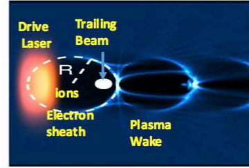
Driven by a laser pulse
