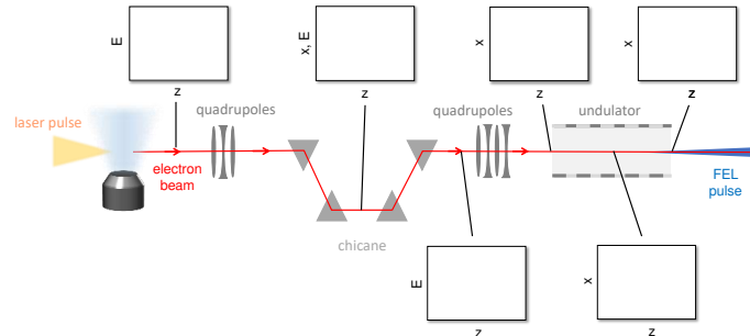
Figure 6 – Schematic of a free electron laser based on a laser-plasma accelerator, using a decompression chicane. At the exit of the laser-plasma accelerator, the electron beam has small bunch length and large energy spread. After the 4 dipoles of the chicane, the bunch is stretched to a longer bunch length, with high energy electrons at the front, low energy electrons at the rear, and a very small slice energy spread. In the undulator, chromatic matching is used so that low energy electrons are focused at the undulator entrance, electrons at the central energy are focused in the middle, and high energy electrons at the end of the undulator, in a way that the FEL radiation slips along the bunch and stays overlapped with the focused part of the electron bunch.
