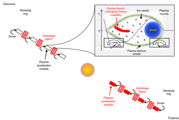
Figure 5 – Schematic of a plasma-based electron-positron collider, highlighting in red some of the key challenges that require basic R&D: namely hosing instability, staging and plasma-based positron acceleration (not exhaustive).
