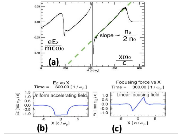
Fig.3: (a) The on axis longitudinal electric field E_z of a wake in the “bubble” regime. The slope of the accelerating field in the first bubble is n_b/2n_0 = \epsilon/2 . (b) The transverse variation of the longitudinal E_z field and (c) transverse variation of the focusing field F_x = (E_x - B_y) . In the bubble regime the E_z field is constant whereas the focusing field is linear in the transverse direction x .
