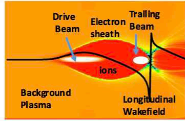
Driven by an electron beam
