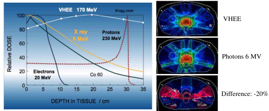
Figure 8 – Radiotherapy with very high energy electrons: (left) depth profiles of dose deposition in tissue for protons, photons, low energy electrons (20 MeV) and very high energy electrons (170 MeV). Comparison between treatment plans with high energy electrons (VHEE) and photons (6 MV). Reproduced with permission from Mutation Research/Reviews in Mutation Research , 704, 142-151 (2010). Copyright 2010 Elsevier.
