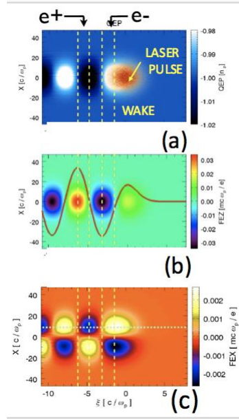
Fig.1 Linear wake excited in an underdense ( n/n_c < 1 ) plasma by laser pulse with a_0=0.1 . The contours of (a) the density disturbance, (b) the longitudinal electric field and the on axis magnitude of this field (black curve) and (c) the transverse focusing force. The two vertical dotted lines show the range of phases of the wake where the wakefield is both accelerating and focusing for electrons ( e^- ) and positrons ( e^+ ) respectively. There is a \pi radians phase difference between the phases available for electron and positron acceleration.
