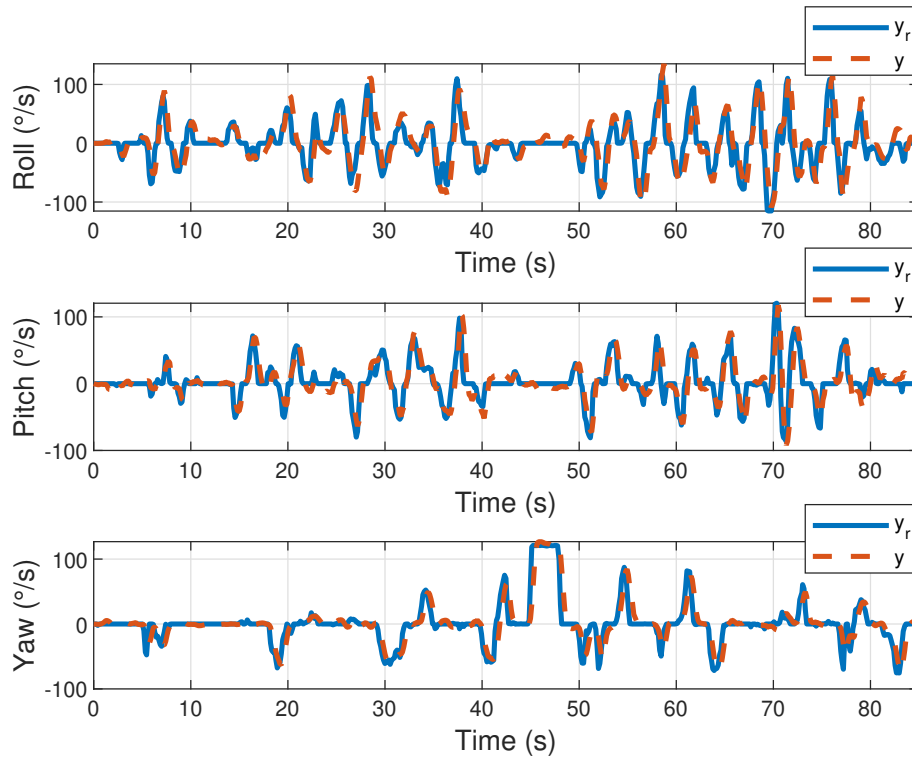
Fig. 3: DJI F450 roll, pitch, and yaw performance.
