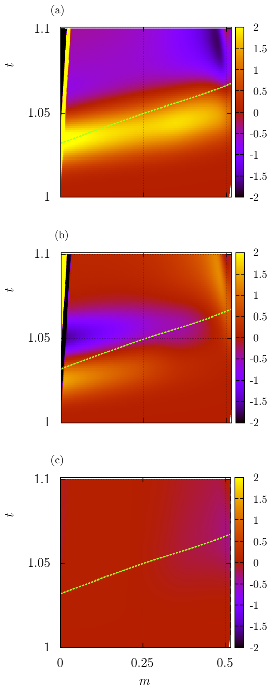
FIG. 10. Contribution from advection, diffusion and remaining terms from Eq. (10a) to the variation rate of \widehat{\mathcal{W}}_1 ( n, k_\perp ) = (4, 1). The dash line represents a \mathcal{C}_1 characteristics trajectory originating from the top of the heat-flux pulse (Eq. 5).
