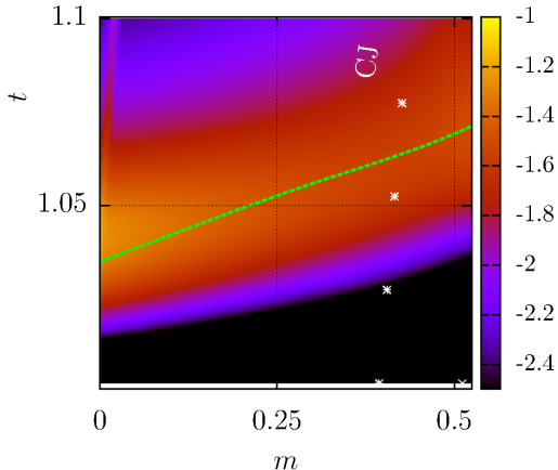
FIG. 2. Projection of the solution to Eq. (4) for a heat flux perturbation (n, k_{\perp}) = (4, 1) on pseudo-characteristic \widehat{\mathcal{W}}_1 in the conduction region in logscale. The dashed line represents a \mathcal{C}_1 characteristics originating from the pulse half height (Eq. 11). Trajectory of the CJ point (*) is also indicated.
