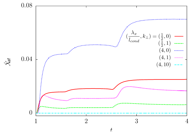
FIG. 9. Deformation of the ablation front \hat{X}_{af} at early times for different longitudinal characteristic \lambda_x/l_{cond} = \{1/2, 4\} and transverse wavenumbers k_{\perp} = \{0, 1, 10\} .
