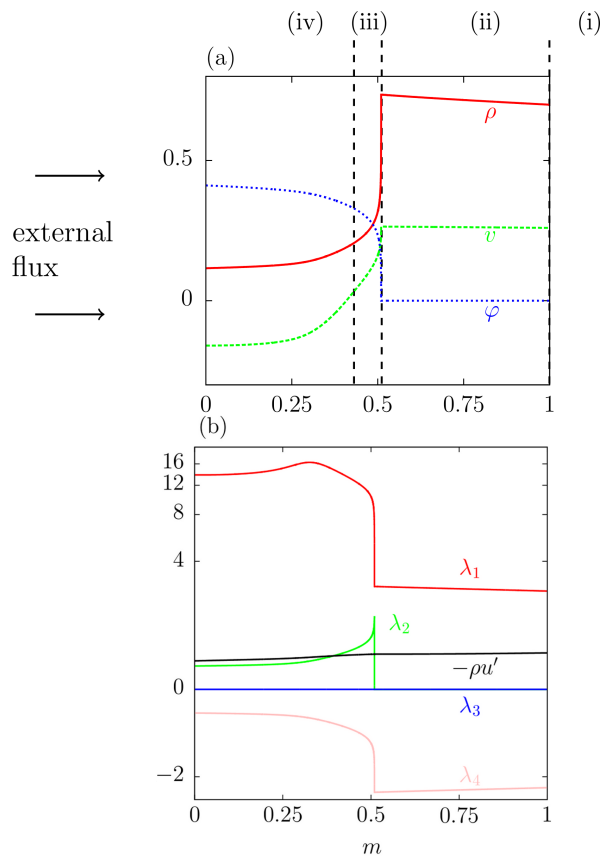
FIG. 1. (a) Base flow profiles in the Lagrangian coordinate m scaled by the function defined by \text{slog}_1(\cdot) \equiv \text{sgn}(\cdot) \log(1 + |\cdot|) . Density ( \rho ), longitudinal velocity ( v ) and heat flux ( \varphi ). (b) Characteristic wave speeds (Eq. 9) ( \lambda_{1,2,3,4} ) and fluid momentum relatively to the ablation front ( -\rho u' ).
