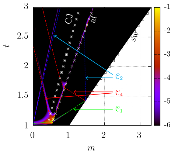
FIG. 7. Baroclinic term (Eq. 12) in logscale for an external heat flux perturbation (n, k_{\perp}) = (4, 1) . Dash lines represent characteristic trajectories as in Fig. 4.
