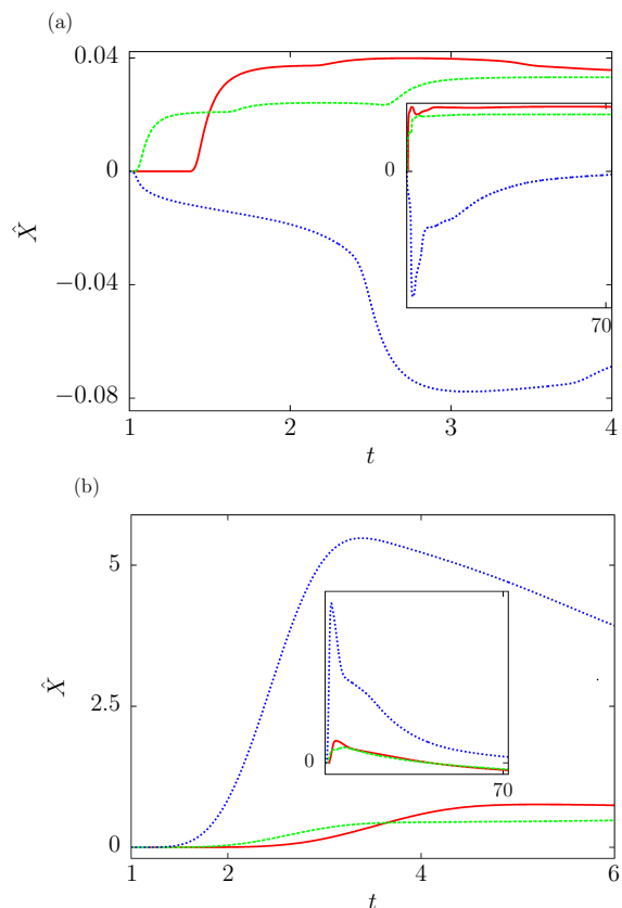
FIG. 8. Deformations of the shock front \hat{X}_{sf} (red, solid), the ablation front \hat{X}_{af} (green, dashed) and the external surface \hat{X}_{es} (blue, dotted) for (a) a longitudinal heat-flux and (b) pressure perturbation (n, k_{\perp}) = (4, 0) , normalized to unity (Eq. 13). These deformations are first order perturbations of mean positions appearing on Fig. 4. The insets illustrate long time behaviours.
