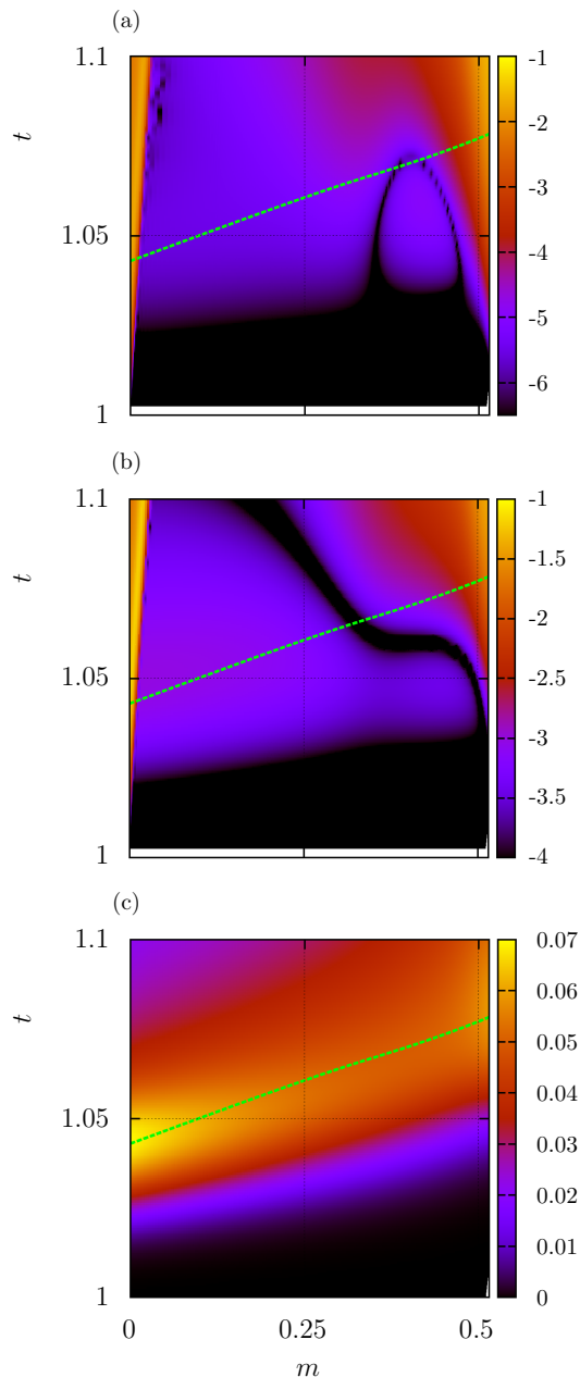
FIG. 3. Perturbation in (a) density in logscale, (b) longitudinal velocity in logscale and (c) temperature in \text{slog}_1 scale, for a heat-flux perturbation with (n, k_{\perp}) = (4, 0) . The dashed line represents a \mathcal{C}_1 characteristics originating from the pulse half height (Eq. 11).
