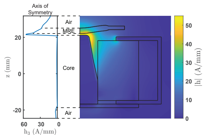
Fig. 10. Eulerian h -field plotted on the xz face and along the axis of symmetry. The field corresponds to an applied current I=2.7 A in the “coil plus core” configuration.
