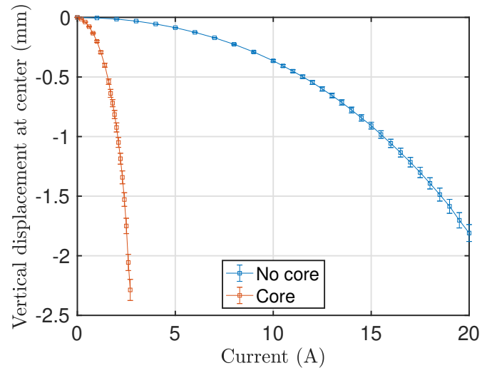
Fig. 4. Influence of the core on the device behavior: vertical position at the center of the upper surface of the disk for a 70 phr ( c=0.08 ) isotropic disk layer in the presence of and in the absence of the core. The reported values correspond to the average over three tests conducted in the same configuration and error bars represent a standard deviation.
