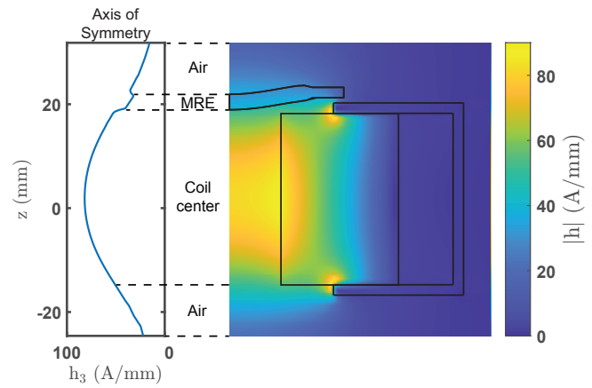
Fig. 8. Eulerian h -field plotted on the xz face and along the axis of symmetry. The field corresponds to an applied current I=20 A in the “coil only” configuration.
