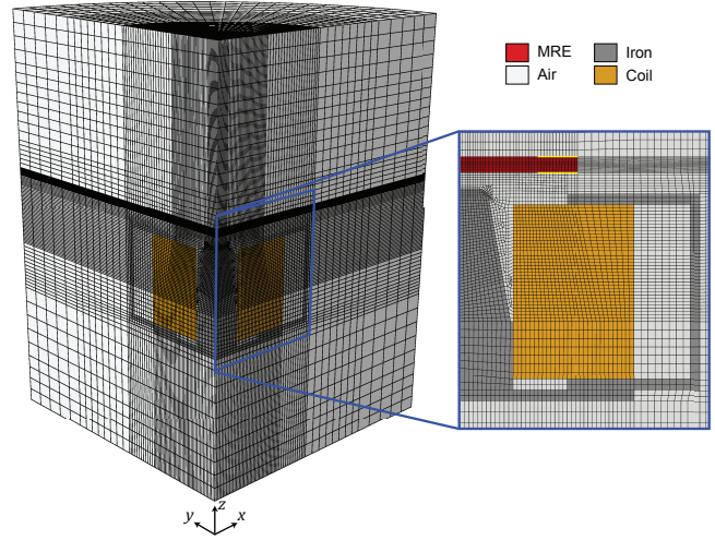
Fig. 5. Finite element mesh for the device configuration with the core present.
