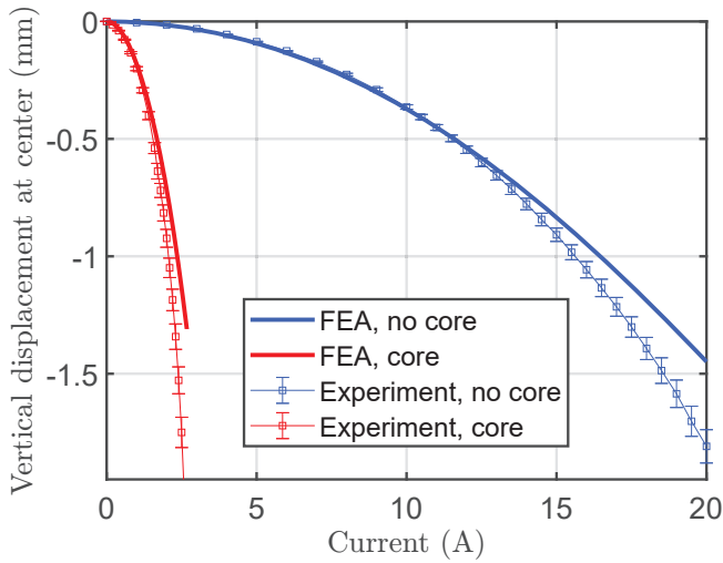
Fig. 6. Comparison between experiments and finite element simulations for device configurations with and without the core: vertical position at the center of the upper surface of the isotropic MRE layer.
