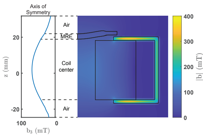
Fig. 7. Eulerian magnetic field b plotted on the xz face and along the axis of symmetry. The field corresponds to an applied current I=20 A in the “coil only” configuration.
