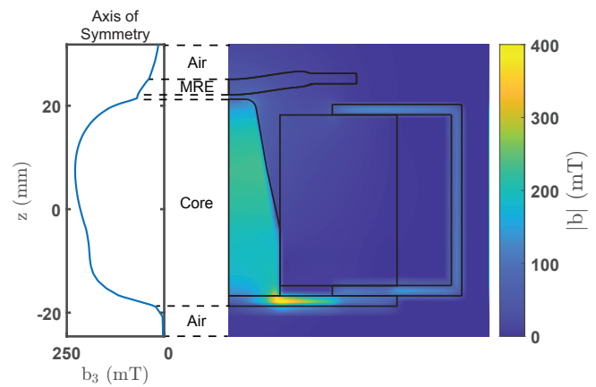
Fig. 9. Eulerian magnetic field b plotted on the xz face and along the axis of symmetry. The field corresponds to an applied current I=2.7 A in the “coil plus core” configuration.
