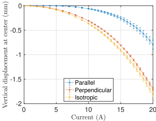
Fig. 3. Effect of particle field-structuring on the device behavior: vertical position at the center of the upper surface of the disk for 70 phr ( c=0.08 ) disk layers that are isotropic, perpendicular and parallel. The reported values correspond to the average over three tests conducted in the same configuration and error bars represent a standard deviation.
