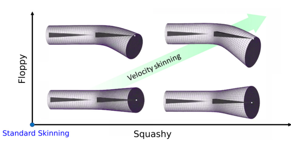
Figure 3: The deformer of squashy and floppy velocity skinning reveal information in the still about the speed and direction of the motion that is not visible in the standard skinning surface.
