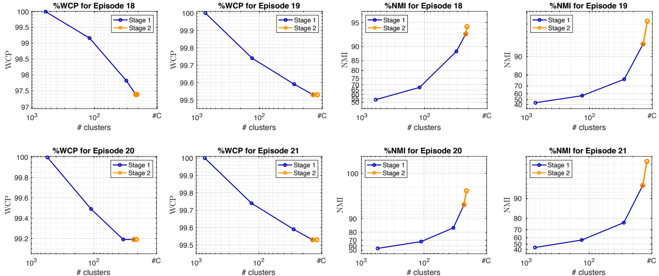
Figure 3: Stage 1 and Stage 2 Person-Clustering results from the program set, Friends. %WCP and %NMI for episodes of Friends from VP CD, for the Automatic Termination protocol (AT). The blue line illustrates the results after Stage 1, while the orange one illustrates the results after Stage 2, i.e. bridging clusters by exploiting the voice modality. #C is the ground truth number of clusters for each episode.
