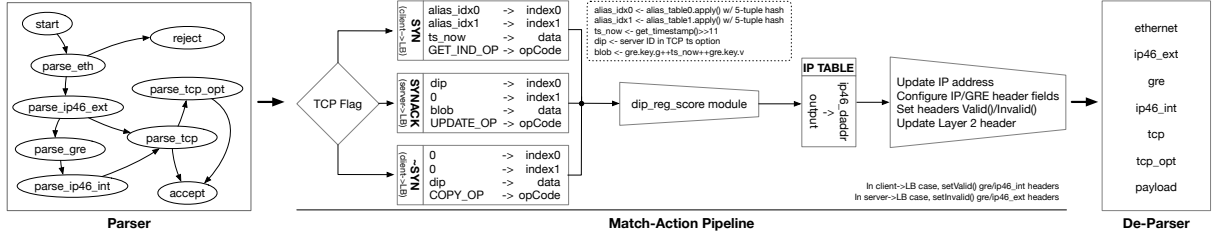
Figure 5. P4 workflow.
