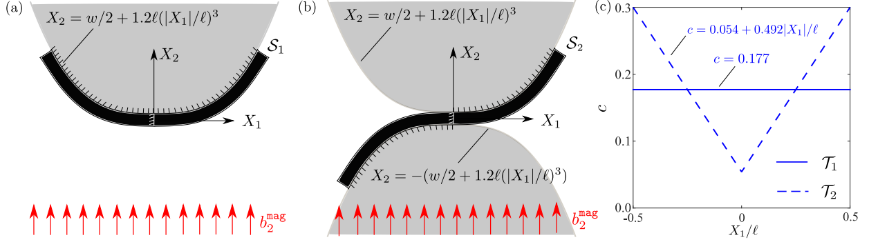
Figure 13: (a,b) Pre-magnetization profiles along the magnetizing field b_2^{\text{mag}} direction for the h -MRE beams of r_{\text{asp}} = 20 . The profile \mathcal{S}_1 in (a) is considered to be the mirror image with respect to X_2 axis, whereas, \mathcal{S}_2 in (b) is considered to be the mirror image with respect to both, X_1 and X_2 . (c) Volume fraction distribution profiles, namely, \mathcal{T}_1 and \mathcal{T}_2 , along the length of the beam.
