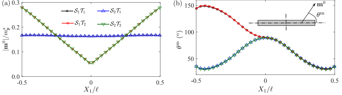
Figure 14: Variation of the remanent magnetization \mathbf{m}^0 (a) magnitudes and (b) directions along the length of the pre-magnetized h -MRE beams of type \mathcal{S}_i\mathcal{T}_i ( i = 1, 2 ).
