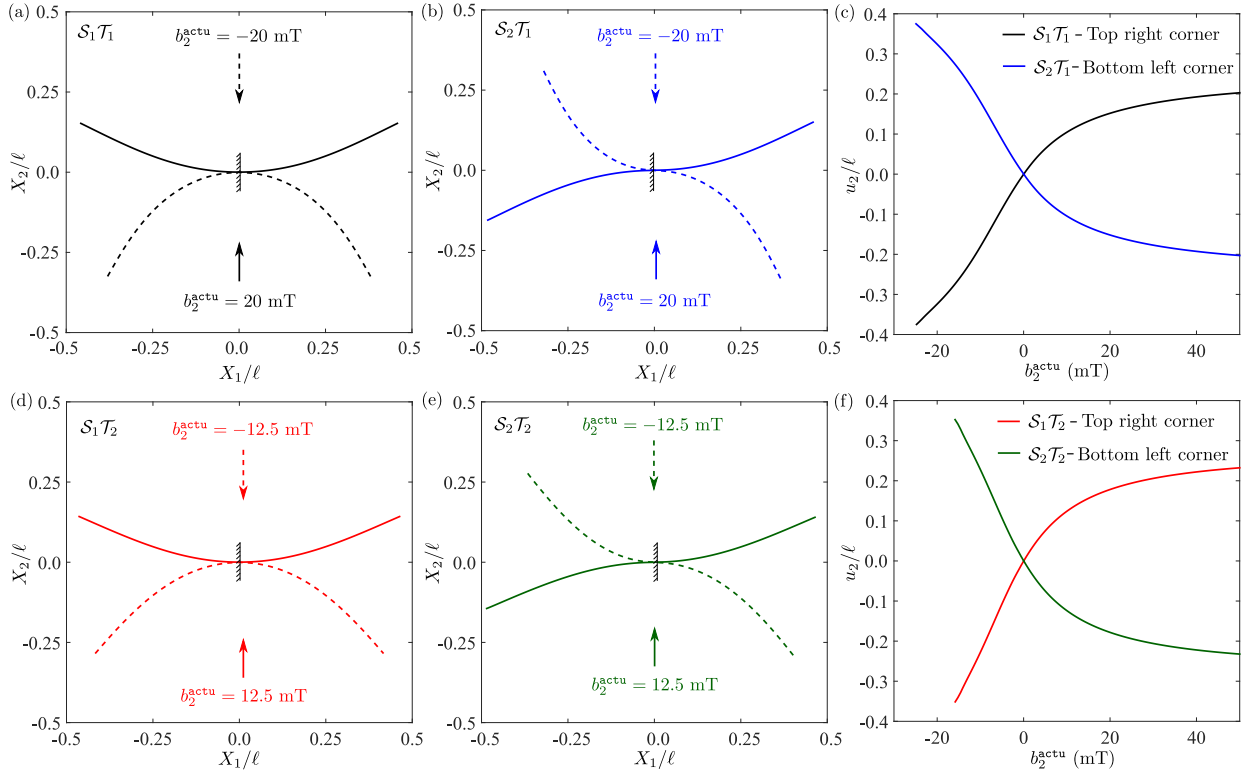
Figure 16: Deflected centerlines of the h -MREs type (a) \mathcal{S}_1 \mathcal{T}_1 and (b) \mathcal{S}_2 \mathcal{T}_1 under the actuation fields b_2^{\text{actu}} = 20 and -20 mT along \hat{\mathbf{E}}_2 . (c) Variation of the top-right corner deflection of \mathcal{S}_1 \mathcal{T}_1 and bottom left corner deflection \mathcal{S}_2 \mathcal{T}_1 under b_2^{\text{actu}} . Deflected centerlines of the h -MREs type (d) \mathcal{S}_1 \mathcal{T}_2 and (e) \mathcal{S}_2 \mathcal{T}_2 under the actuation fields b_2^{\text{actu}} = 12.5 and -12.5 mT along \hat{\mathbf{E}}_2 . (f) Variation of the top-right corner deflection of \mathcal{S}_1 \mathcal{T}_2 and bottom left corner deflection \mathcal{S}_2 \mathcal{T}_2 under b_2^{\text{actu}} .
