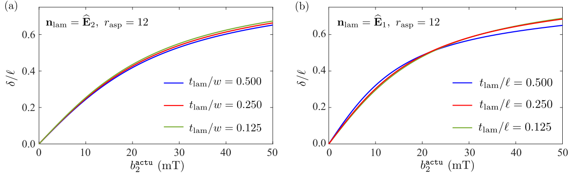
Figure 11: End-tip deflection of the cantilevered h -/ s -MRE laminates with overall r_{\text{asp}} = 12 and (a) \mathbf{n}_{\text{lam}} = \hat{\mathbf{E}}_2 , (b) \mathbf{n}_{\text{lam}} = \hat{\mathbf{E}}_1 under the actuation field b_2^{\text{actu}} along \hat{\mathbf{E}}_2 . Effect of a decreasing t_{\text{lam}} on the end-tip deflections are shown.
