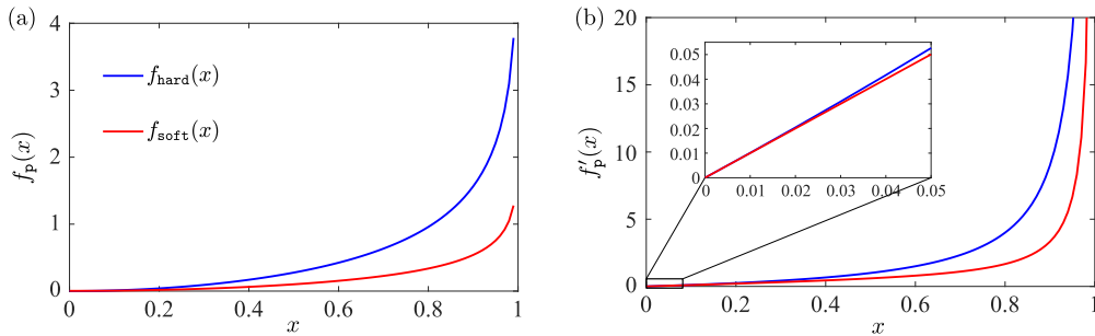
Figure 3: Comparison of the (a) hardening functions f_p(x) and (b) their derivatives f'_p(x) for the hard and soft magnetic particles.
