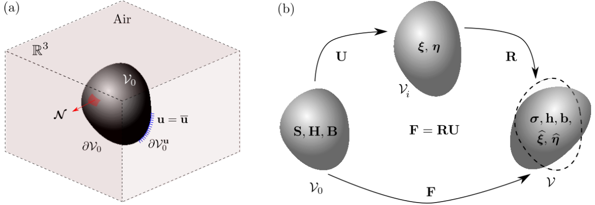
Figure 1: (a) Reference configuration of the h -MRE of volume V_0 and boundary \partial V_0 along with the surrounding air, occupying a volume \mathbb{R}^3 \setminus V_0 . (b) Definition of the reference, intermediate and current configurations of volume V_0 , V_i and V , respectively, along with the different field variables defined therein.
