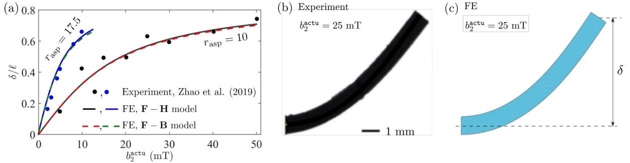
Figure 7: (a) Comparison of the experimentally measured and the model (both F – H and F – B ) predicted end-tip deflections of the pre-magnetized cantilever beams of r_{\text{asp}} = 10 and 17.5 under the applied actuation field along \mathbf{e}_2 . Comparison of the FE predicted deflected beam shape with the respective experimental measurements of Zhao et al. (2019) under b_2^{\text{actu}} = 25 mT for (b) r_{\text{asp}} = 10 and (c) 17.5.
