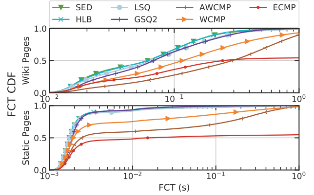
Figure 8. [Testbed] FCT CDF comparisons for two types of requests in the 24-hour Wikipedia replay.
