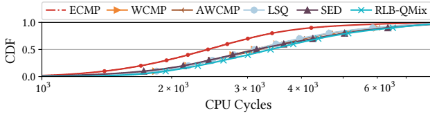
Figure 11: Load balancing decision making latency for each network flow measured under 800 flows/s traffic rate.
