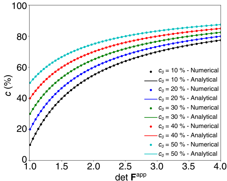
Figure 15: Evolution of porosity c = 1 - \rho as a function of the applied determinant of the deformation gradient, as obtained by numerical simulations and the analytical expression (A.9).
