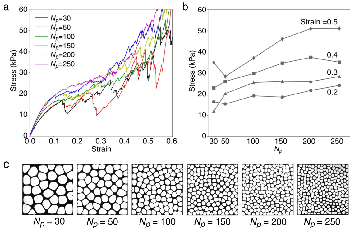
Figure 6: Experimental representativity study for M-Voronoi with \rho = 0.3 in terms of number of voids N_p . (a) Stress-strain response of the M-Voronoi with different number of voids and (b) engineering stress as a function of N_p for different levels of the overall strain. (c) Optical images of the corresponding realizations for different N_p .
