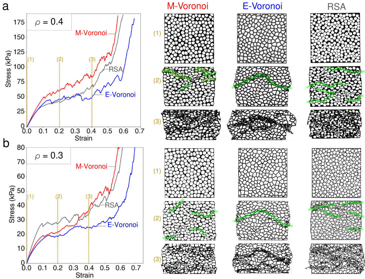
Figure 10: Compression experiments and corresponding optical images for the M-Voronoi, E-Voronoi and RSA geometries for relative densities (a) \rho = 0.4 and (b) \rho = 0.3 . For all cases, snapshots are shown of the three geometries selected at three intermediate strains levels, denoted with (1), (2) and (3). The green lines indicate zones of strong localization and fracturing of the intervoid ligaments. The in-plane dimensions of the undeformed specimens are 100 \times 100 \text{ mm}^2 . (For interpretation of the references to color in this figure legend, the reader is referred to the web version of this article.)
