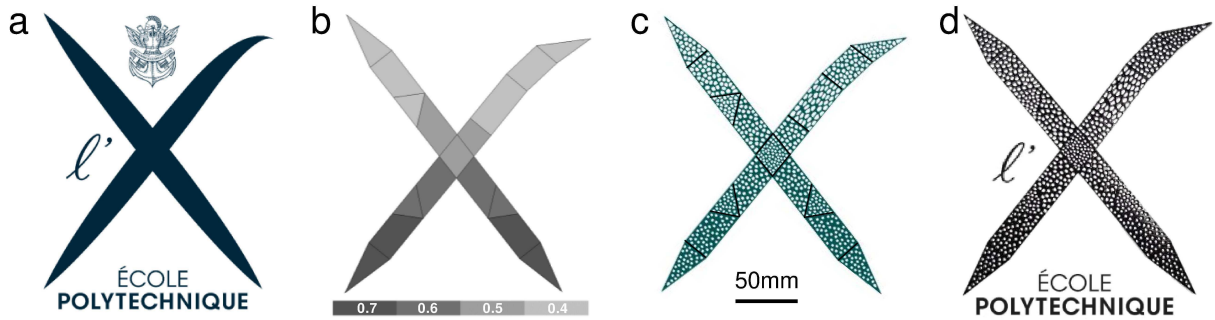
Figure 14: Assembly of individual M-Voronoi cells into a macroscopic geometry. (a) Ecole Polytechnique Logo. (b) Finite Volume Element (FVE) discretization with arbitrary porosity and anisotropy. (c) Numerical creation and assembly of the individual porous cells. (d) 3D-printed specimen.
