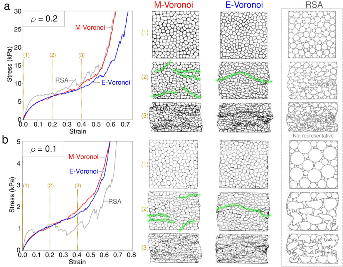
Figure 11: Compression experiments and corresponding optical images for the M-Voronoi, E-Voronoi and RSA geometries for different relative densities (a) \rho = 0.2 and (b) \rho = 0.1 . For all cases, snapshots are shown of the three geometries selected at three intermediate strains levels, denoted with (1), (2) and (3). The green lines indicate zones of strong localization and fracturing of the intervoid ligaments. The RSA for \rho = 0.2, 0.1 are non-representative due to fabrication limitations. The in-plane dimensions of the undeformed specimens are 100 \times 100 \text{ mm}^2 . (For interpretation of the references to color in this figure legend, the reader is referred to the web version of this article.)
