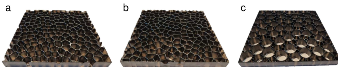
Figure 5: (a) M-Voronoi, (b) E-Voronoi and (c) RSA 3D-printed specimens with no interruption strategy and \rho = 0.2 .
