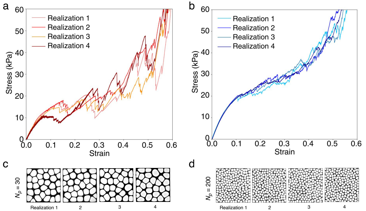
Figure 7: Experimental representativity study for M-Voronoi with \rho = 0.3 in terms of number of realizations and number of voids. Stress-strain response for four different realizations for (a) N_p = 30 and (b) N_p = 200 . Corresponding optical images of the realizations for (c) N_p = 30 and (d) N_p = 200 .
