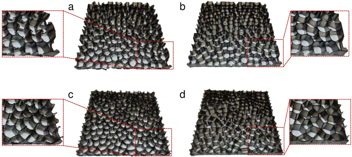
Figure 4: (a,b) M-Voronoi and (c,d) E-Voronoi 3D-printed specimens with relative density \rho = 0.1 . The specimens are obtained in (a,c) without and (b,d) with the interruption strategy.
