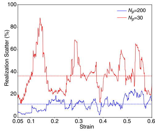
Figure 8: The scatter in the stress-strain response induced by four different realizations of M-Voronoi geometries with \rho = 0.3 and number of voids N_p = 30, 200 . The straight dotted lines indicate the average value over the strain range considered in the figure.
