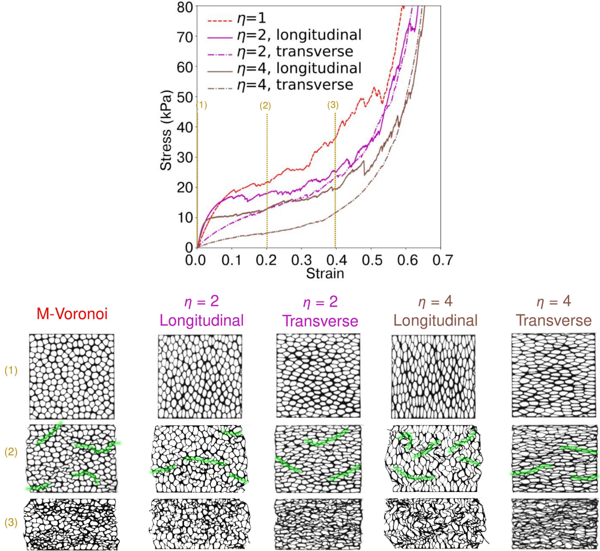
Figure 13: Compression experiments and corresponding optical images for the isotropic and anisotropic M-Voronoi along the longitudinal and transverse direction for \rho = 0.3 . For all cases, snapshots are shown of the three relevant geometries selected at three intermediate strains levels, denoted with (1), (2) and (3). The green lines indicate zones of strong localization and fracturing of the intervoid ligaments. The in-plane dimensions of the undeformed specimens are 100 \times 100 \text{ mm}^2 . (For interpretation of the references to color in this figure legend, the reader is referred to the web version of this article.)
