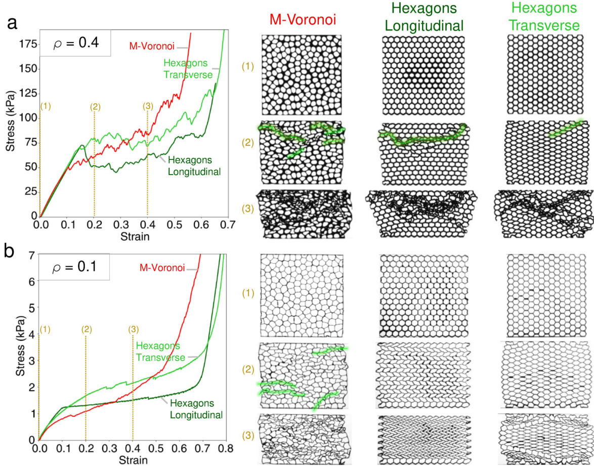
Figure 12: Compression experiments and corresponding optical images for the M-Voronoi, Honeycombs along the longitudinal and transverse direction for two relative densities (a) \rho = 0.4 and (b) \rho = 0.1 . For all cases, snapshots are shown of the three relevant geometries selected at three intermediate strains levels, denoted with (1), (2) and (3). The green lines indicate zones of strong localization and fracturing of the intervoid ligaments. The in-plane dimensions of the undeformed specimens are 100 \times 100 \text{ mm}^2 . (For interpretation of the references to color in this figure legend, the reader is referred to the web version of this article.)
