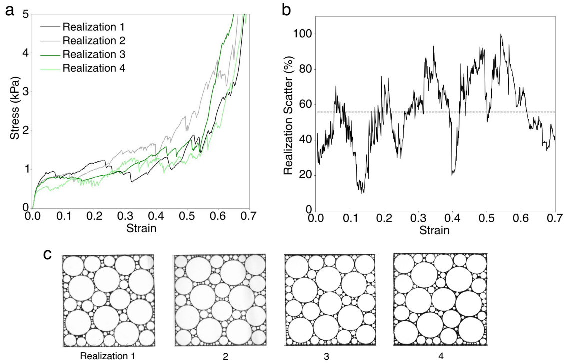
Figure 9: Experimental representativity study for RSA with \rho = 0.1 in terms of number of realizations. (a) Stress-strain response for four different realizations. (b) Stress-strain realization scatter. The straight dotted line indicates the average value over the strain range considered in the figure. (c) Corresponding optical images of the realizations considered.
