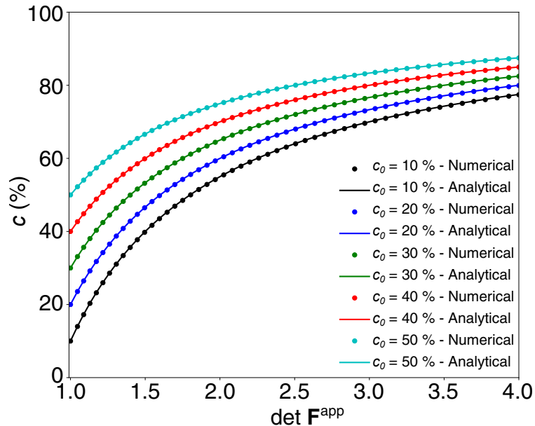
Figure 15: Evolution of porosity c = 1 - \rho as a function of the applied determinant of the deformation gradient, as obtained by numerical simulations and the analytical expression (A.9).
