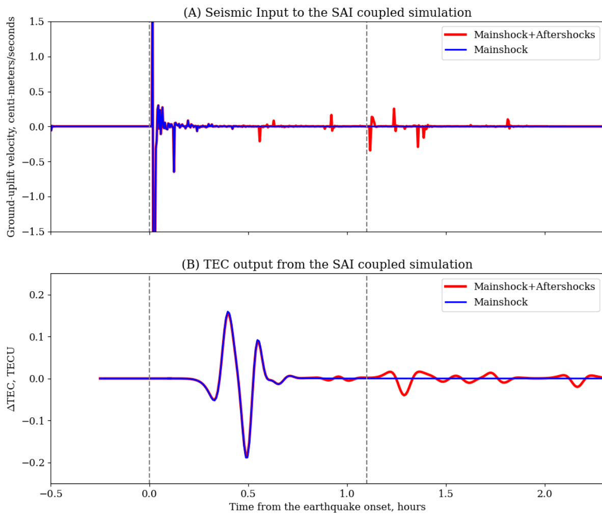
Figure A3. Simulation results from the SAI coupling model: (A) the ground vibration at the epicenter with and without the aftershocks. (B) simulated \Delta\text{TEC} with and without aftershocks.
