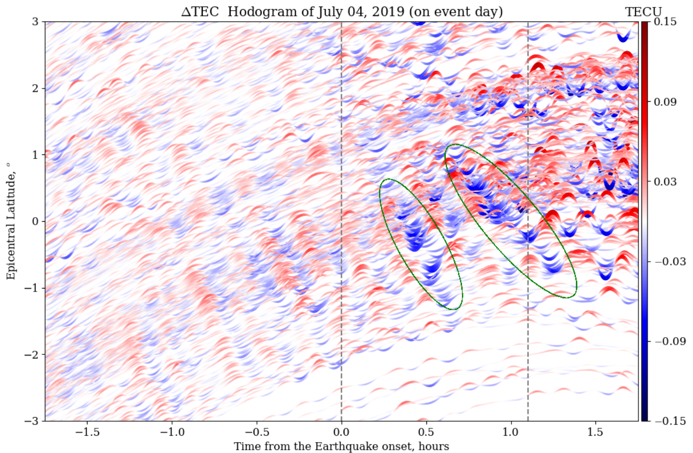
Figure 6. Hodogram of observed \Delta\text{TEC} on the earthquake day.
