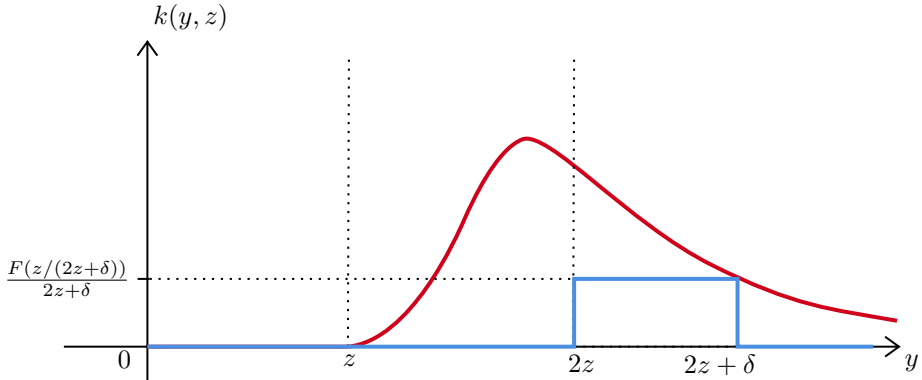
Fig. 3 Example of minorisation for k(a, y, z) = \frac{1}{y} F\left(\frac{z}{y}\right) \mathbb{1}_{z \leq y} and F given by the probability density function of a Beta distribution. Then we have k(a, y, z) > \varepsilon(z) \mathbb{1}_{y \in D(z)} as required by Assumption 1-(v), with |D(z)| = \delta for all z .
