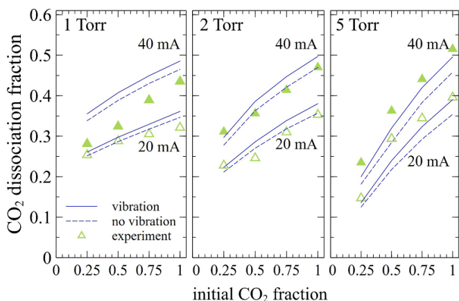
Figure 11. \text{CO}_2 dissociation fraction of a \text{CO}_2\text{-O}_2 discharge as a function of the \text{CO}_2 initial fraction in the \text{CO}_2\text{-O}_2 mixture at 20 mA and 40 mA: experiment ( \Delta ), model calculations by excluding (---) and including (—) the vibrational kinetics. No error bars are included in this figure, since the fitting error of the FTIR spectra and the reproducibility error of the experimental results are smaller than the size of the symbols.
