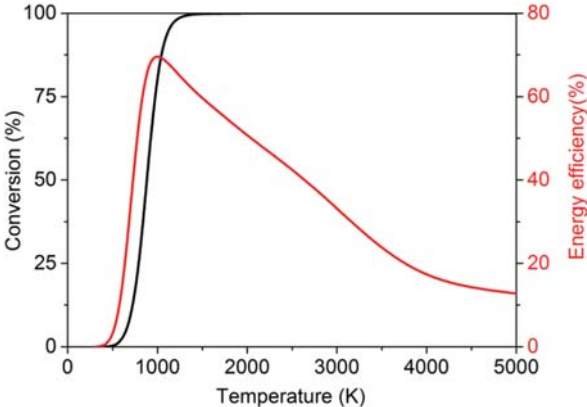
Figure 24 Chemical equilibrium conversion and energy efficiency for dry reforming of CH 4 . Reproduced from [6] with permission from the Royal Society for Chemistry.
