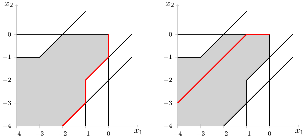
Figure 8.1: Tropical central paths on the Hardy polyhedron (8.7) for the objective function \min x_1 (left) and \min tx_1 + x_2 (right).
