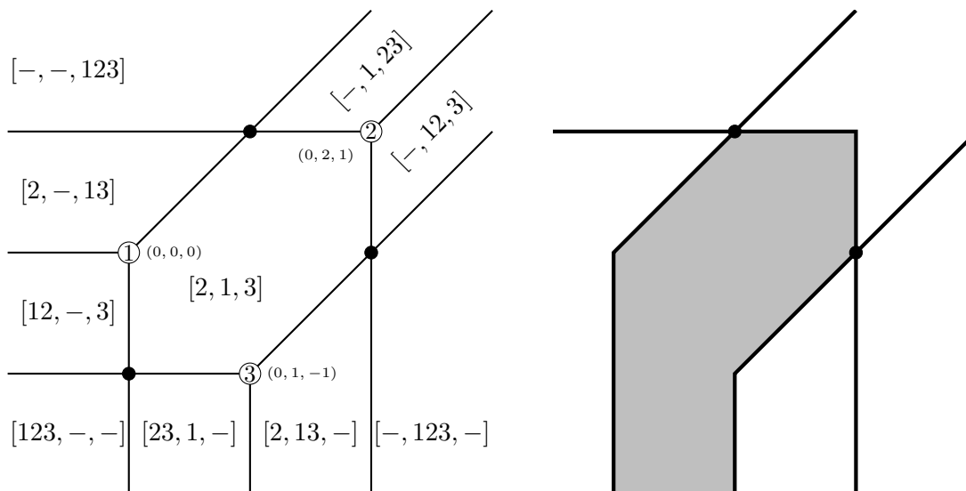
Figure 4.6: Unsigned (left) and signed (right) cell decompositions induced by the three tropical s-hyperplanes in Example 4.23.
