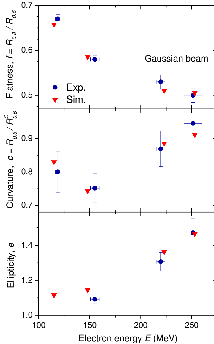
Figure 5.15: Variation of the flatness f , the curvature c and the ellipticity e with the electron energy. The dots corresponds to experimental data (already shown in Fig. 5.11(d,e,f)) and the triangles to simulations. Error bars indicate the standard error of the mean.
