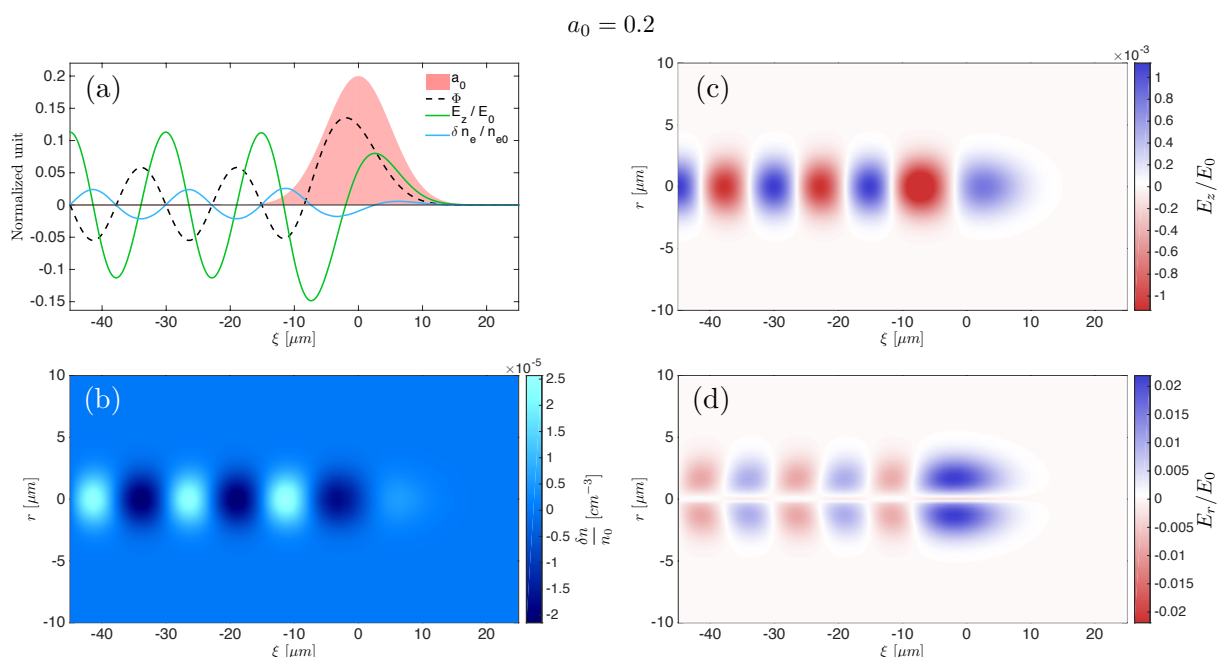
Figure 1.4: Linear wakefield quantities for a_0 = 0.2 : (a) Normalized laser amplitude a , plasma potential \varphi , longitudinal electric field E_z/E_0 and density perturbation \delta n_e/n_{e0} on axis in the co-moving coordinate system. Colormaps of the two-dimension plasma density perturbation \delta n_e(r, \xi)/n_{e0} (b), longitudinal electric field E_z(r, \xi)/E_0 (c) and radial electric field E_r(r, \xi)/E_0 (d).
