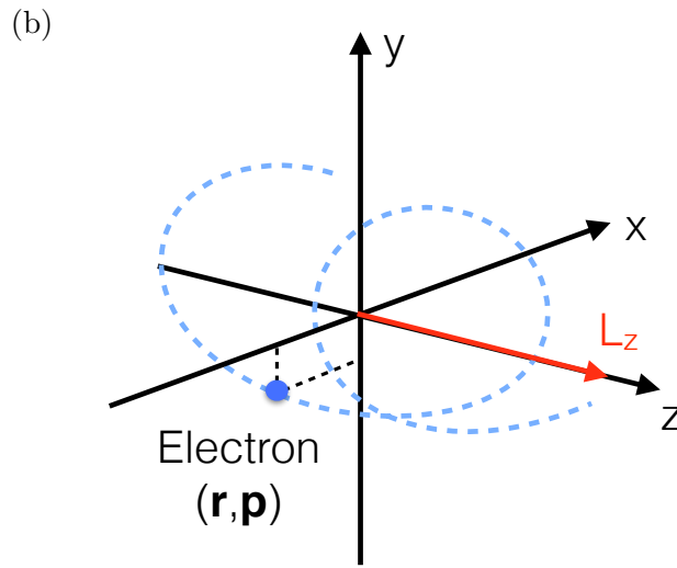
Figure 5.1: Definition of the angular momentum of an electron L_z .
