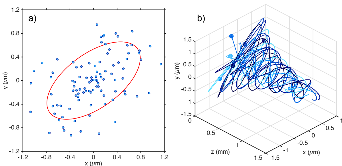
Figure 5.13: (a) Initial transverse distribution of the electron beam for test-particle simulations. (b) Electron orbits for 8 particles along 1.5 mm of acceleration.
