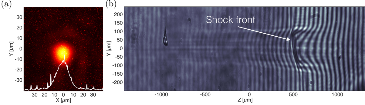
Figure 4.6: (a) Experimental laser focal spot obtained with a 700 mm focal length off-axis parabola. (b) Interferogram of the propagation of the laser in a pure helium gas jet. Z = 0 \text{ mm} corresponds to the center of the nozzle. The shock is visible at z_s = 500 \mu\text{m} .
