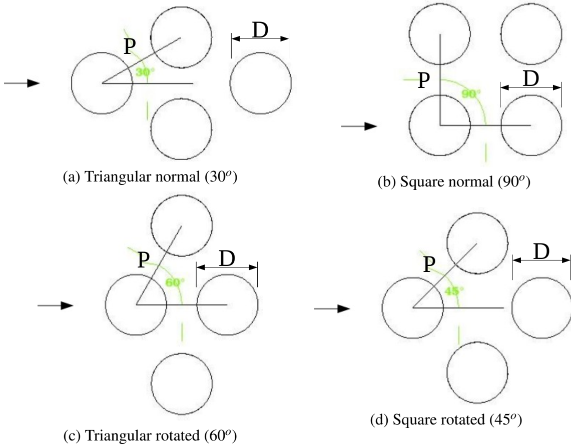
Figure 1.13 Array Configurations.
