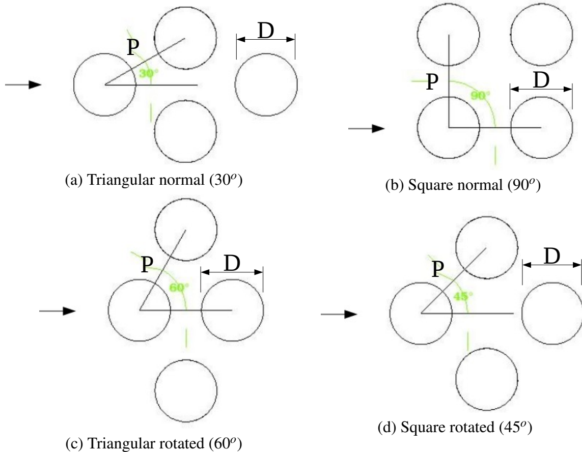
Figure 1.13 Array Configurations.
