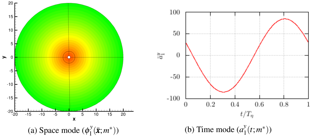
Figure 7.4 The pair of first POD mode of the mesh deformation in y direction at Re = 100 , m^* = 2.50 .
