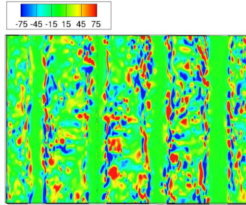
(c) X vorticity ( \omega_x ) at plane L2
