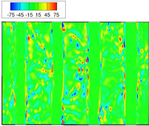
(b) X vorticity ( \omega_x ) at plane L1
