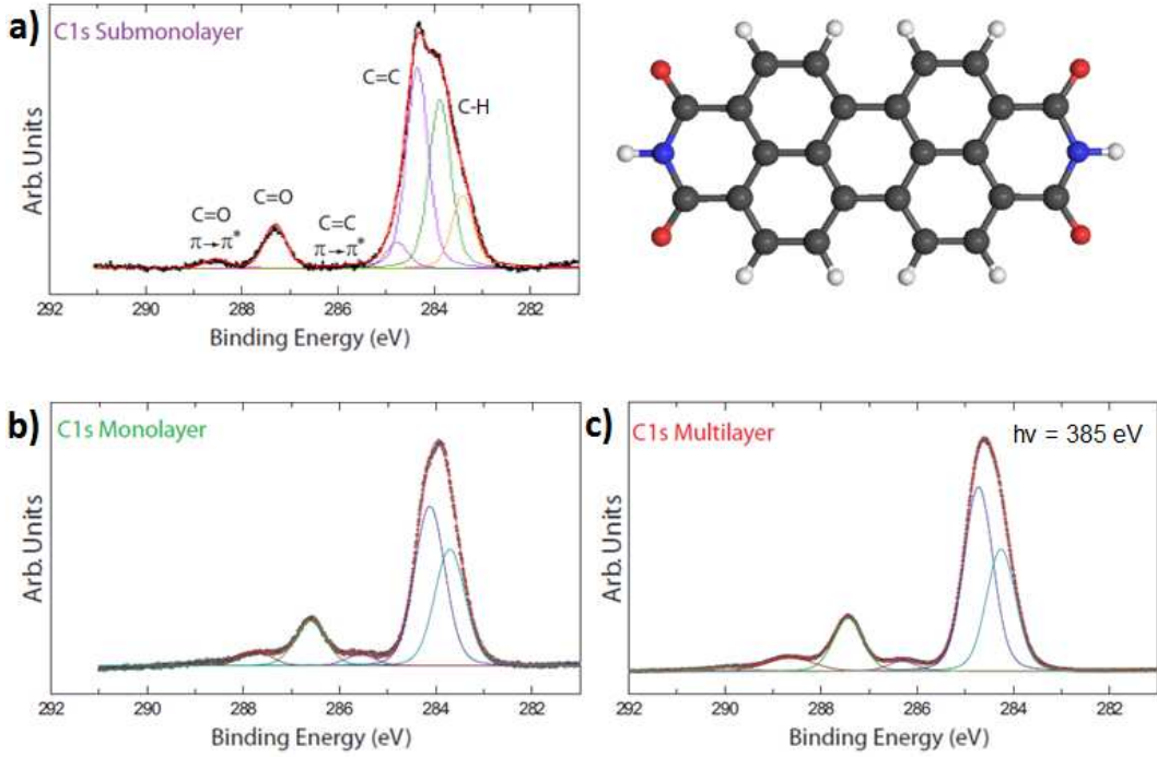
Figure 3.7: PTCDI C 1s core level photoemission spectra measured by using a photon energy h\nu = 385 eV. The PTCDI films were grown on the Au(111) surface with three different coverages: (a) sub-monolayer, (b) monolayer, and (c) multilayer.
