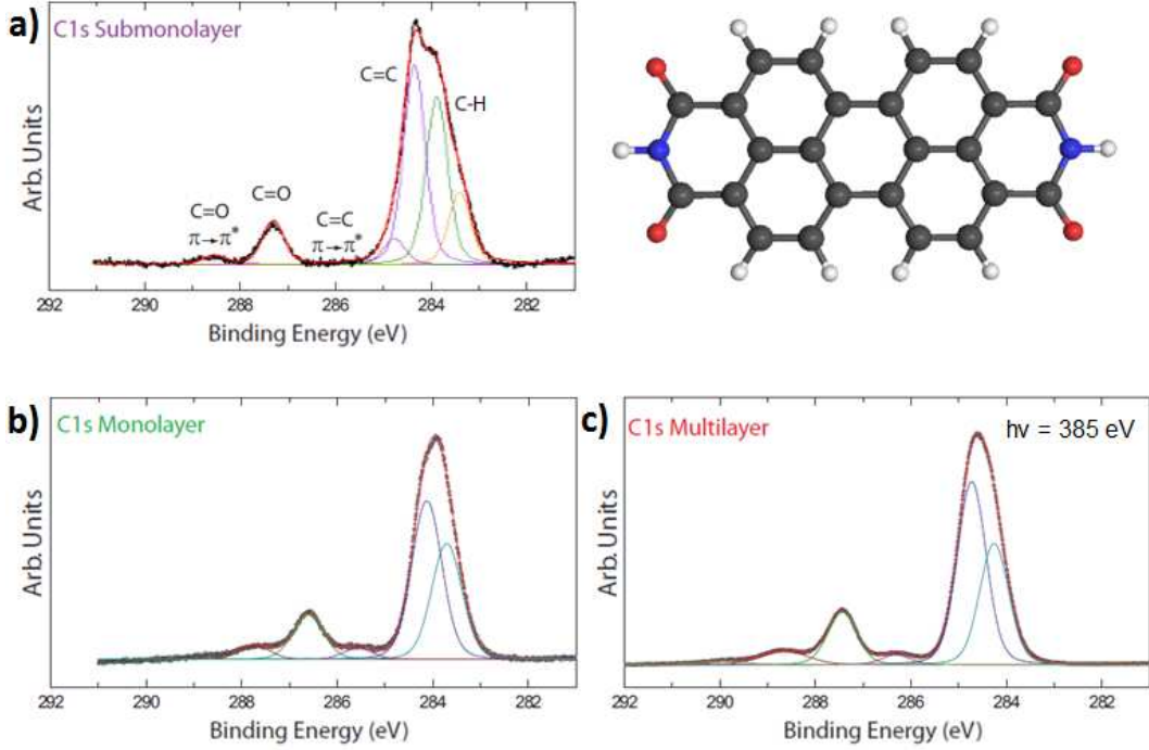
Figure 3.7: PTCDI C_{1s} core level photoemission spectra measured by using a photon energy h\nu = 385 eV. The PTCDI films were grown on the Au(111) surface with three different coverages: (a) sub-monolayer, (b) monolayer, and (c) multilayer.
