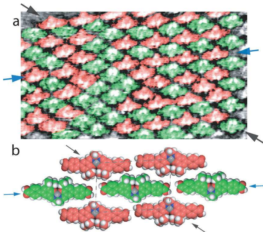
Figure 5.3: (a) STM image of the self-assembled complex 1 nanoarchitecture, 20 \times 11 \text{ nm}^2 ; V_s = 0.8 \text{ V} , I_t = 35 \text{ pA} . Molecules are colored in red or green false color according to their respective orientation. Blue arrows indicate the direction of complex 1 H-bonded chains. Black arrows indicate complex 1 closest-neighbor separation, [143].
