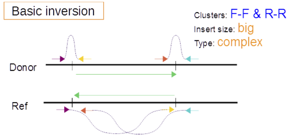
Figure 7.7: Basic inversion.
