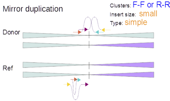
Figure 7.6: Mirror duplication.
