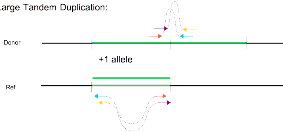
Figure 6.1: Large tandem duplication. One genomic copy is gained in-between two breakpoint positions.
