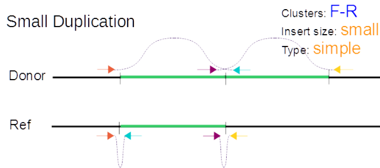
Figure 7.4: Small duplication
