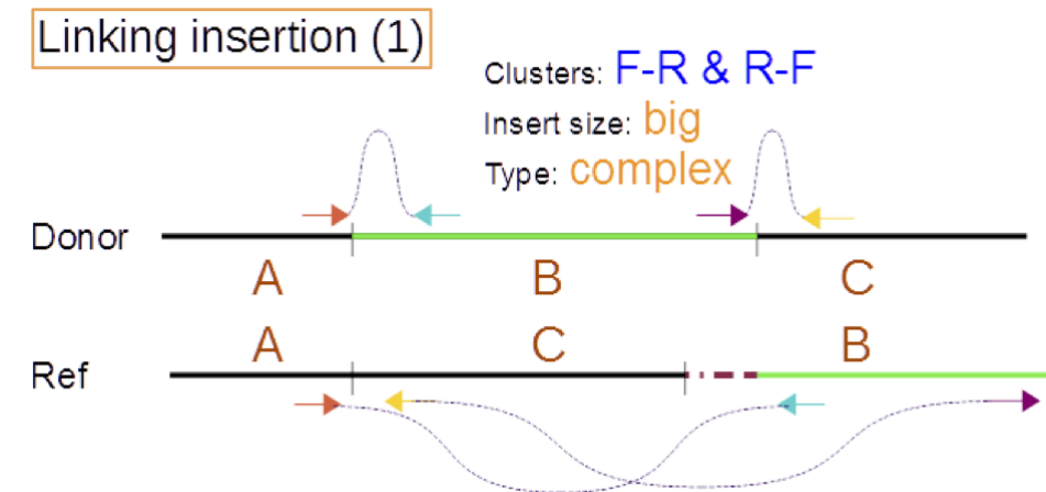
Figure 7.12: Linking insertion.
