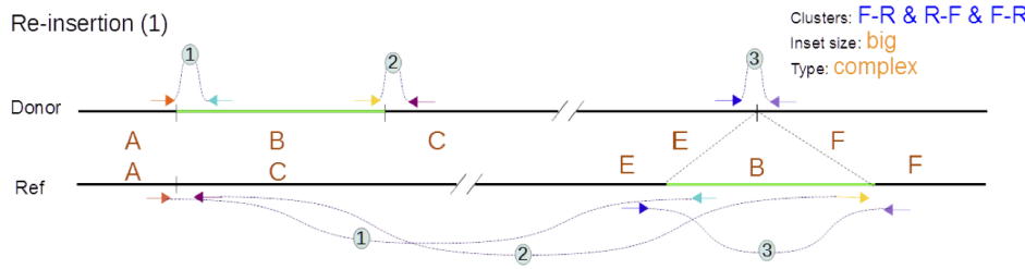
Figure 7.8: Re-insertion.
