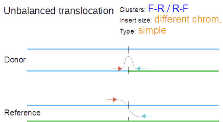
Figure 7.2: Unbalanced translocation
