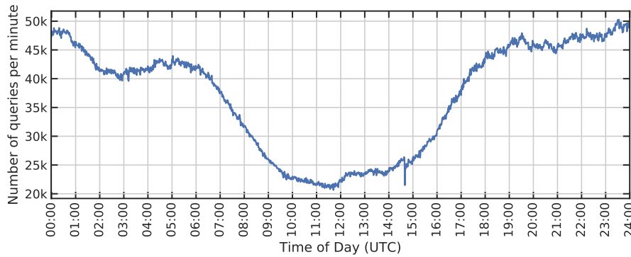
Figure 3.12: Wikipedia 24 hour replay network trace.
