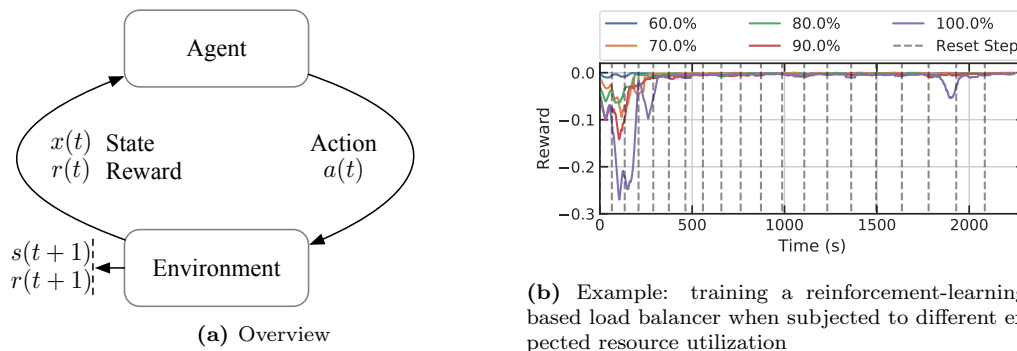
Figure 1.15: Reinforcement learning
