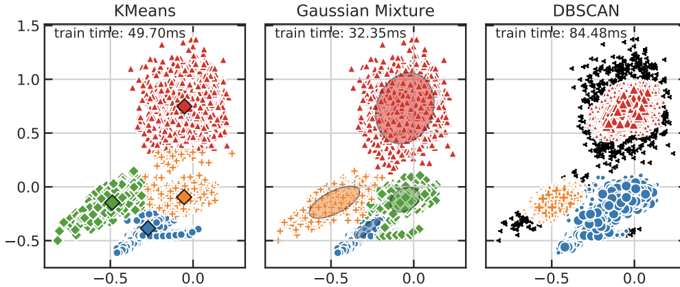
Figure 3.19: Unsupervised clustering using 25 features.
