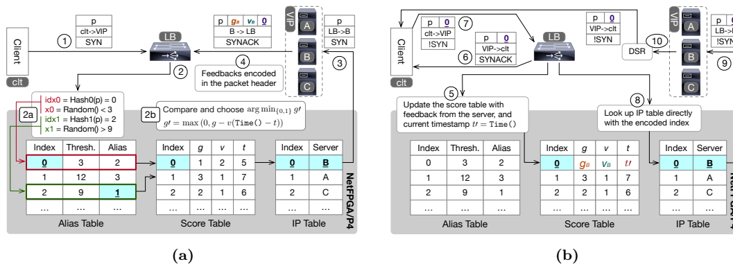
Figure 4.2: Charon overview.
