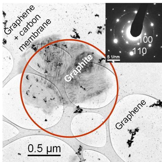
Fig. 4: TEM plan view of graphene and graphite flakes. Sample implanted with the 8-GL dose, annealed at 900^{\circ}\text{C} for 30 min, slowly cooled to 725^{\circ}\text{C} , then quenched. The EDP of the circled area (inset) exhibits 100 and 110 graphite reflections with perfect single crystal order together with 100 and 110 rings; the former correspond to the large graphite crystal in the image and the latter to the surrounding nanocrystalline graphene.
