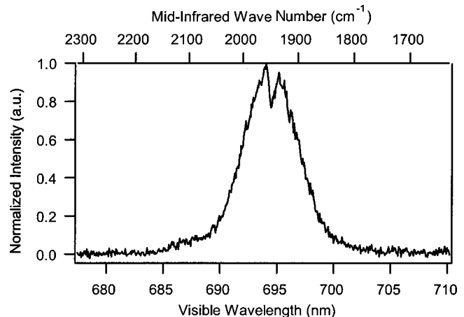
Fig. 2. Spectrum of mid-IR pulses after transmission through 5 mM of a solution of HbCO in a D 2 O buffer solution. The frequency axis was shifted to the center of the peak of the absorption feature at 1951\ \text{cm}^{-1} .
