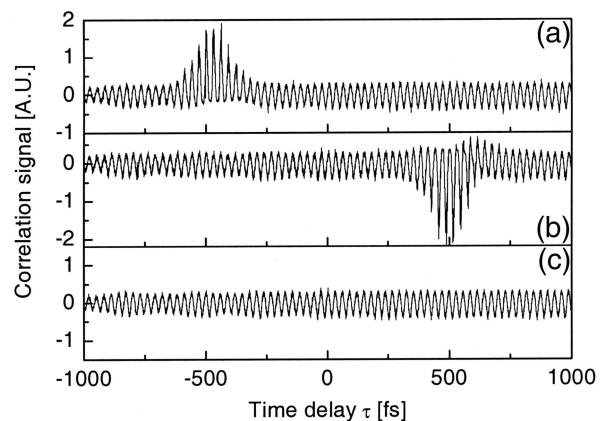
Fig. 2. Correlation function \Delta S_T^{(2)}(\tau) measured for three values of delay T . T_b - T_a = 990 fs, corresponding to frequency shear \delta\omega = 0.97 THz. T_c is chosen such that the pulse replica E(t - T_c) does not overlap the stretched pulse E_S(t) . Note that the fact that (a) points up and (b) points down is fortuitous: In (a) the short pulse E(t - T) and the stretched pulse happen to interfere constructively during their overlap, whereas in (b) they interfere destructively. This effect depends on the exact choice of T and has no influence on the retrieved spectral phase.
