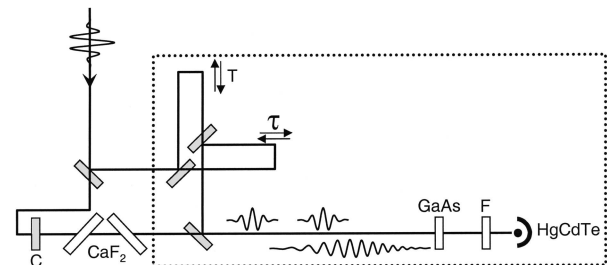
Fig. 1. Experimental setup for time-domain HOT SPIDER, based on a second-order collinear autocorrelator (area inside the dotted box). Second-harmonic generation is achieved in a GaAs crystal of 100- \mu\text{m} thickness and collected with a HgCdTe detector after transmission through a 2–6- \mu\text{m} bandpass filter (F). Scanning of time delay \tau is achieved with a 2-Hz shaker and a copropagating He–Ne laser for accurate length calibration. To transform this standard autocorrelator into a time-domain HOT SPIDER apparatus we add two beam splitters, an optical chopper (C), and two tilted \text{CaF}_2 windows, thus generating the additional stretched pulse.
