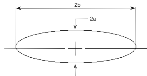
Fig. 4. Model of a Paramecium as an ellipse.
