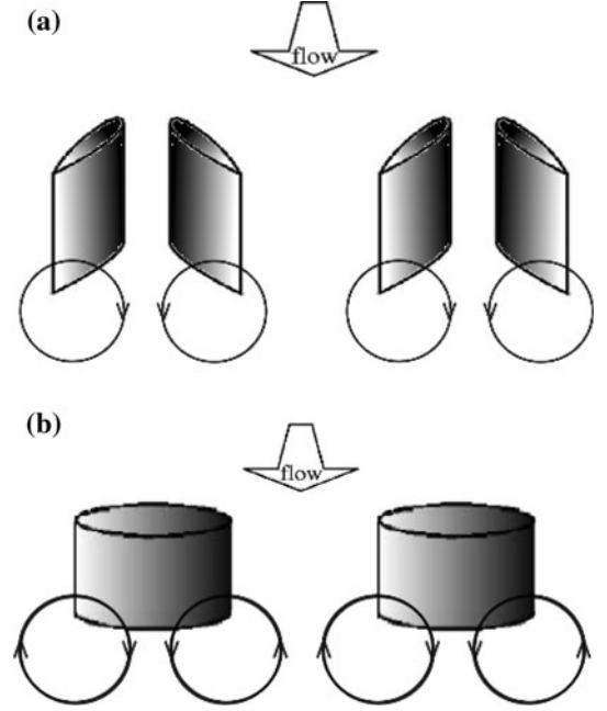
Fig. 1 Sketch of CtR vortices a with common inflow generated by VGs. b interacting with their two neighbors resulting in common inflow and common outflow motions (lift-up effect)
