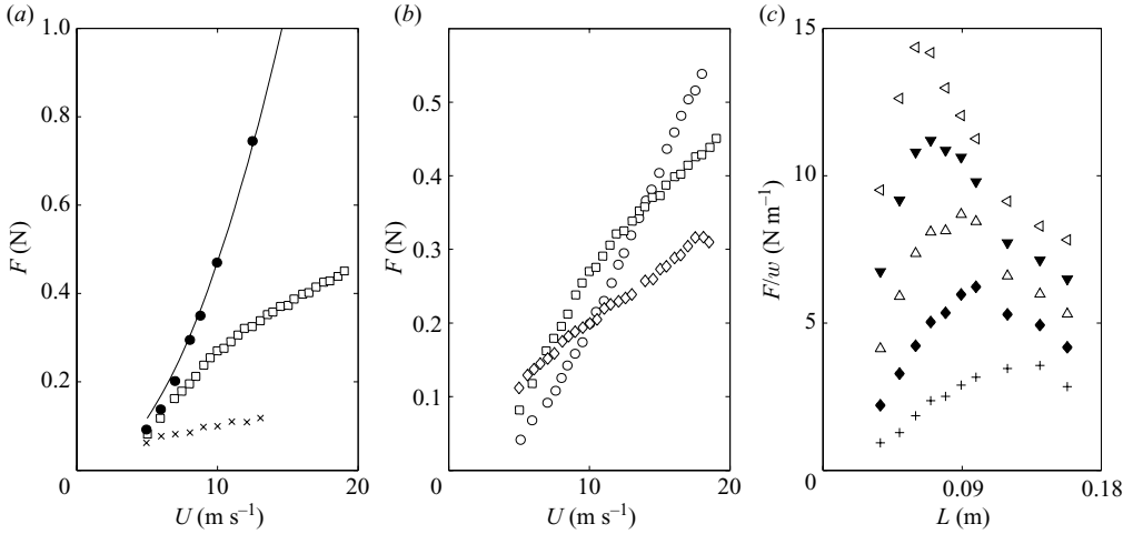
FIGURE 4. Effect of different parameters on the drag of a rectangular plate. (a) Effect of the flexural rigidity on the variation of drag with flow velocity on 10 cm \times 3.8 cm specimens: ( \times ), R16; ( \square ), R7; ( \bullet ), rigid; (—), the fit of the drag of the rigid specimen using (2.1). (b) Effect of the length on the variation of drag with flow velocity: ( \circ ) R3; ( \square ), R7; ( \diamond ), R9. (c) Variation of the drag per unit of width with the length of the specimen. The drag data were obtained by linearly interpolating the drag-versus-velocity data for the following flow velocities: (+), 6 m s -1 ; ( \blacklozenge ), 9 m s -1 ; ( \triangle ), 12 m s -1 ; ( \blacktriangleleft ), 15 m s -1 ; ( \blacktriangleleft ), 18 m s -1 . A detailed listing of the tested specimens is given in the Appendix.
