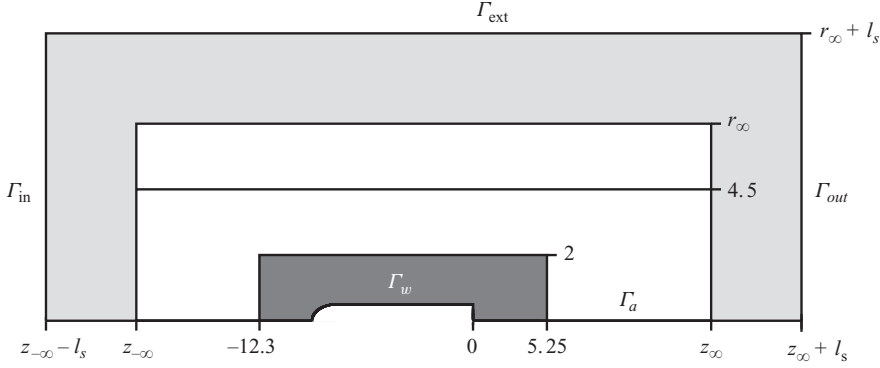
FIGURE 2. Schematic of the computational domain \Omega for the afterbody flow: z_{-\infty} , z_{\infty} and r_{\infty} denote the location of the physical inlet, outlet and lateral boundaries. This physical domain is padded with a sponge zone of width l^s , shown as the light grey shaded area. The inner solid lines delimit regions characterized by different vertex densities. The dark grey shaded area corresponds to the near-wake domain \Omega_{in} used to normalize the eigenmodes.
