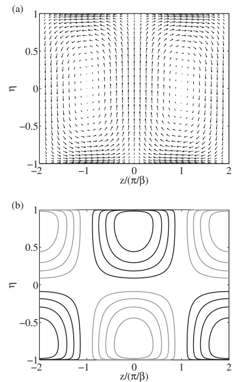
FIG. 3. Transverse view of the optimal solution corresponding to the primary peak ( \lambda_z=4h ) for Re_\tau=5000 : (a) represents the initial ( v, w ) field ( t=0 ); (b) represents the optimal streamwise velocity streaks obtained in response to this perturbation at t=t_{\max} . The black contours are high velocity streaks u>0 and the gray contours are low velocity streaks u<0 . The levels are 0.2(+0.2)0.8 .
