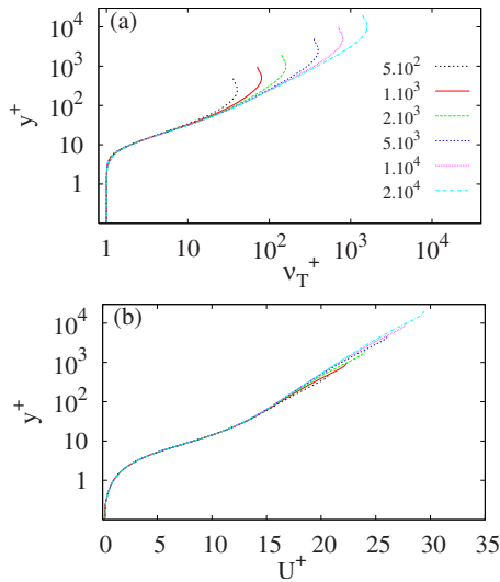
FIG. 1. (Color online) (a) Cess eddy viscosity \nu_T^+ and (b) corresponding mean velocity profile, both displayed in wall units for the selected Reynolds numbers \text{Re}_\tau = 500, 1000, 2000, 5000, 10\,000 , and 20\,000 .
