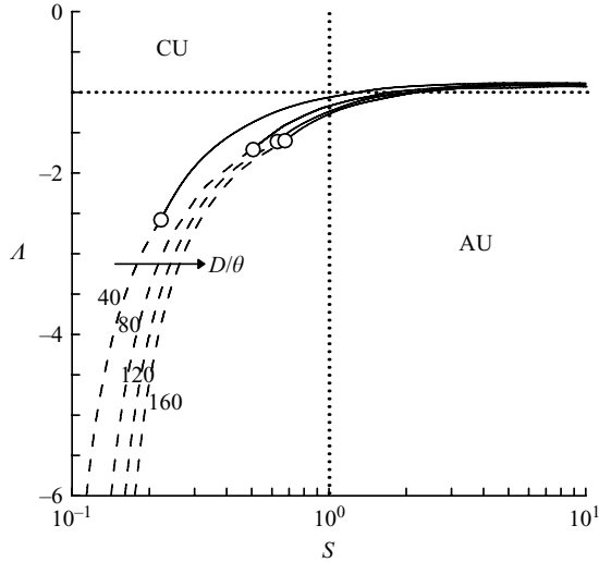
FIGURE 11. Boundary separating the regions of absolute (AU) and convective (CU) instability and crossover points ( \circ ) in the (S, A) -plane for the steepness parameters 40, 80, 120 and 160, at M_\infty = 0 and Re_\infty = 2000 (---, SLM_0 ; —, WM_1 ).
