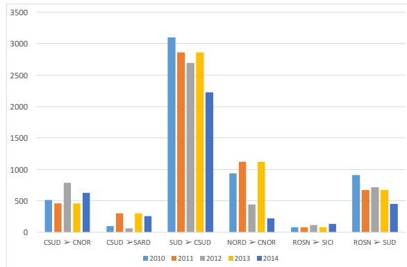
Figure 7: Average physical exchanges between the zones
