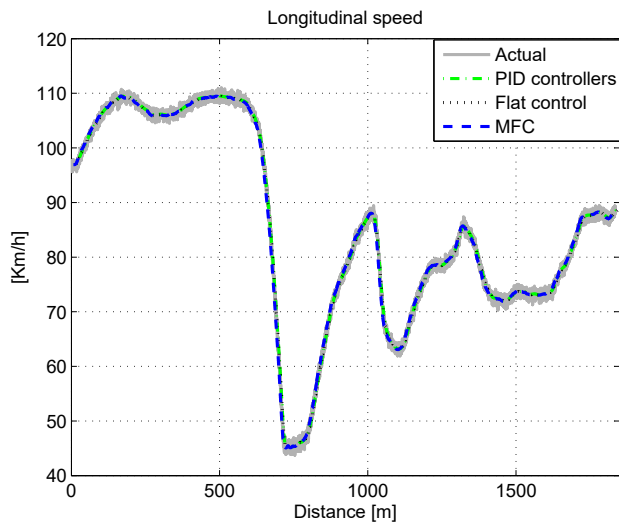
Fig. 6. The actual longitudinal speed versus the closed-loop simulated longitudinal velocities
