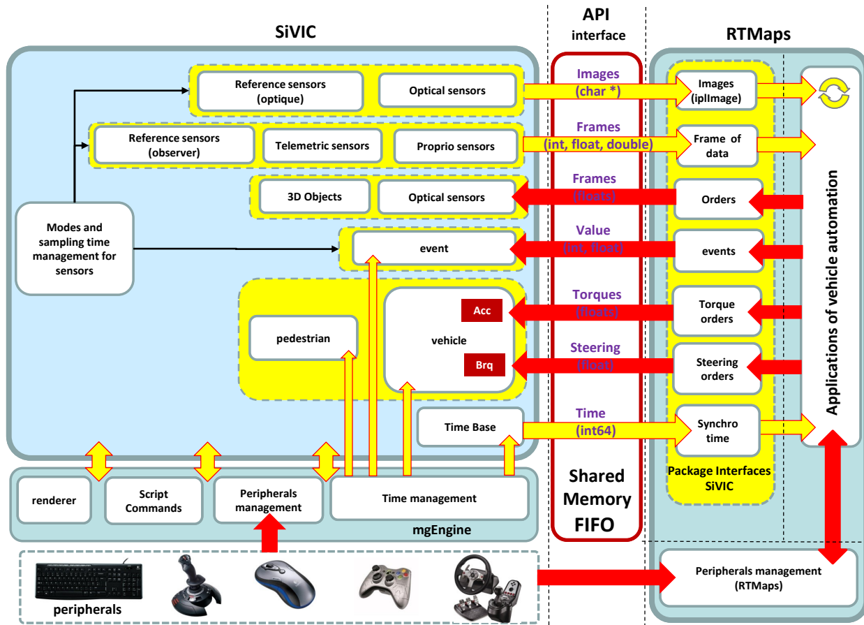
Fig. 11. SiVIC/Types of data managed between pro-SiVIC and RTMaps
