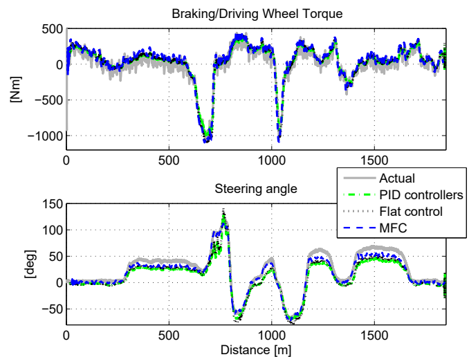
Fig. 8. Wheel torques and steering angles control signals: actual and simulated
