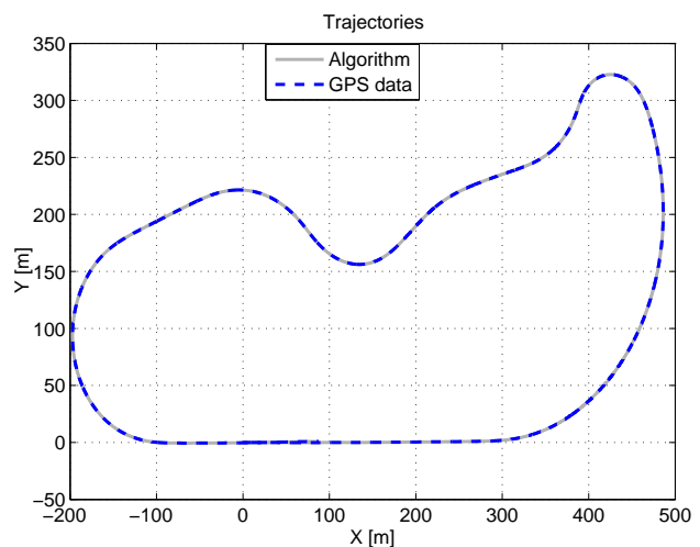
Fig. 3. GPS trajectory and trajectory of the algorithm (20)
