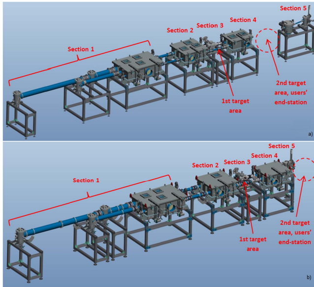
Figure 6. Layout of the two GHHG HR beamlines: (a) GAS, the diagnostic section is in-line; (b) CONDENSED, the diagnostic section is in-line (the spectral diagnostics if off-line).
