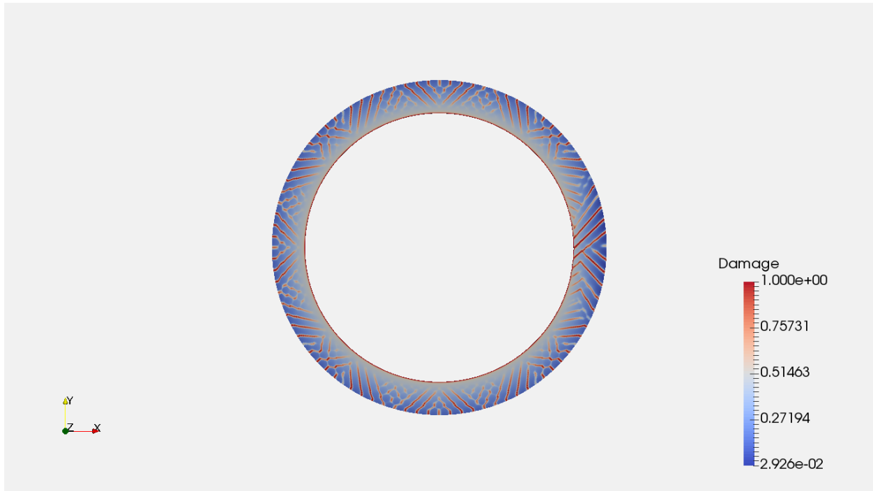
Figure 16: Damage profile for a ductile material and smaller characteristic length.
