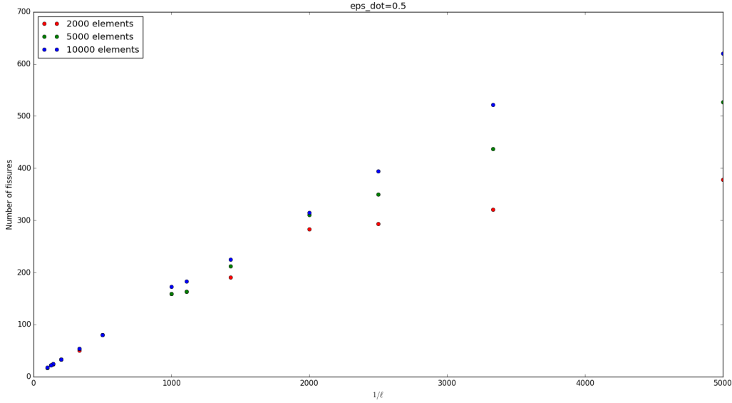
Figure 11: We see that the number of cracks is almost proportional to 1/\ell if the mesh is fine enough. In here, \dot{\epsilon}_0 = 0.5
