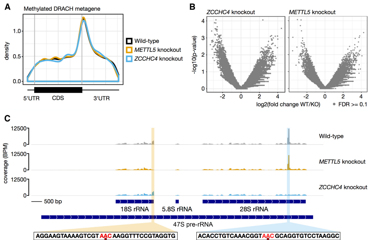
Figure 4. Transcriptome-wide mapping of m 6 A by miCLIP reveals that METTL5 and ZCCHC4 are exclusively ribosomal RNA writers. (A) Metagene analysis of all m 6 A sites identified on mRNAs. The called m 6 A sites in each replicate were collapsed and plotted with the MetaPlotR pipeline (75). This shows the typical distribution of m 6 A, with enrichment at the stop codon and a high degree of overlap between the different conditions. DRACH, m 6 A modification consensus motif (D = A, G or U; R = A or G; H = A, C or U). (B) No other sites in the transcriptome are methylated by METTL5 or ZCCHC4. Coverage in sliding windows across each transcript was calculated and normalized per transcript. Differential bins between wild-type and each knockout were tested for significance with edgeR and plotted as a volcano plot. No sites in the transcriptome passed the false discovery rate (FDR) threshold of 0.1, indicating that no mRNA adenosines are methylated by METTL5 or ZCCHC4. (C) The genome track for the 47S pre-rRNA locus confirms that METTL5 and ZCCHC4 are the writers for m 6 A on the 18S and 28S rRNAs, respectively. C-to-T transitions are the most frequent substitution at m 6 A sites caused by antibody cross-linking. As both the 18S and 28S m 6 A marks are in a AAC context (red in the sequence shown below; the m 6 A is indicated by a red dot), reads were filtered for those containing CT to reduce background at this locus. The peaks for the 18S m 6 A and the 28S m 6 A (highlighted) are lost, respectively, in the mettl5 - and zcchc4 -knockout cells. The miCLIP sequencing data is available on the Gene Expression Omnibus database (accession number GSE128699).
