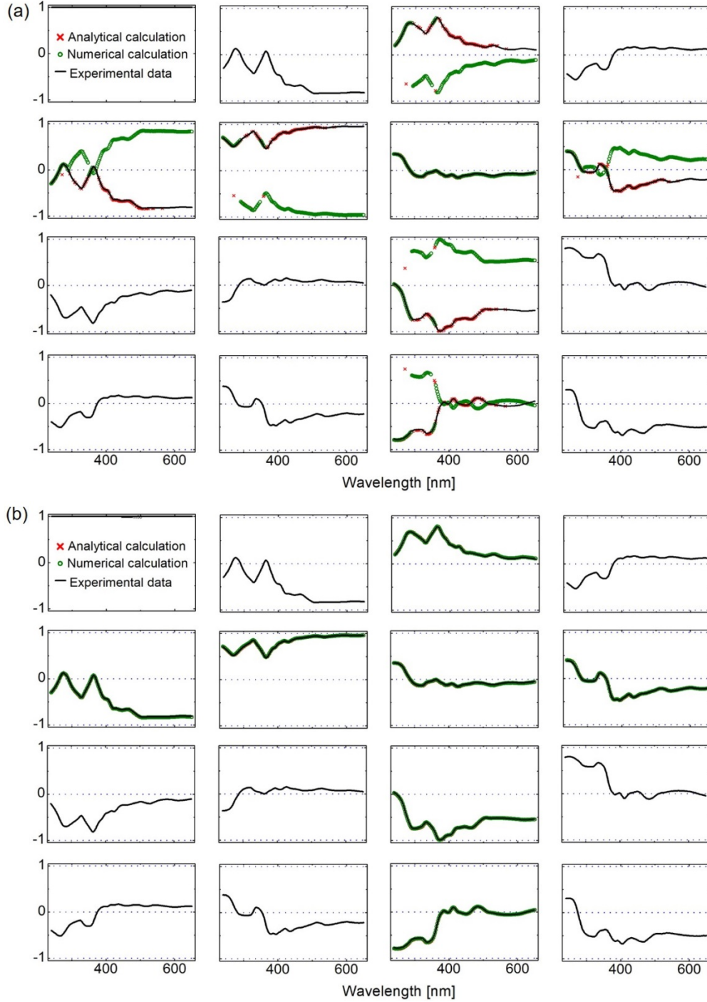
Fig. 1. (a) Complete Mueller matrix of the grating (solid line) and its recovery from a partial \mathbf{M}(2, 3) by using the analytical procedure from Appendix B (red crosses) and the numerical approach (green circles). (b) Complete and recovered Mueller matrices assuming weak anisotropy or exploiting symmetry.
