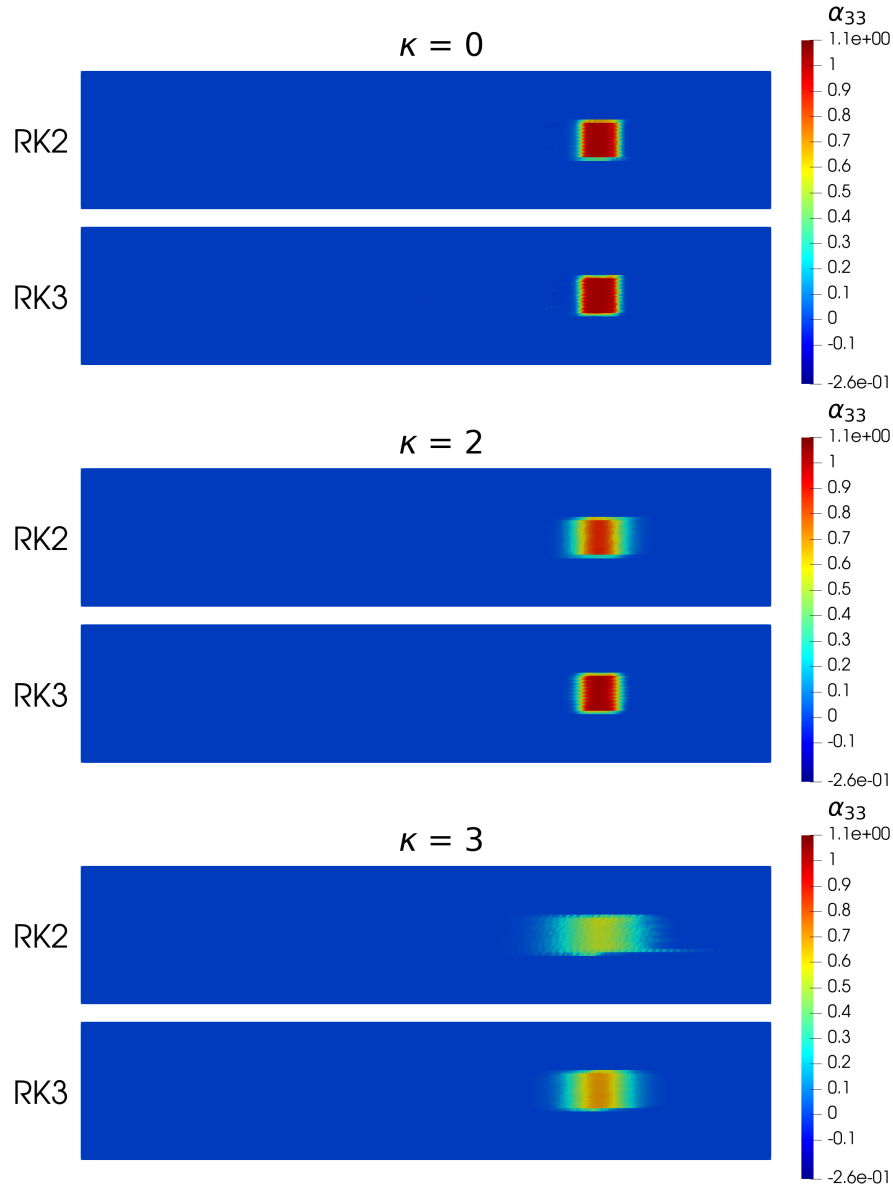
Figure 5: Role of upwinding penalty : Comparison between the final states predicted by the RK2 and the RK3 schemes for different upwinding penalties \kappa = 0, 2, 3 for the transport of a single screw dislocation with density \alpha_{33} \text{ nm}^{-1} (initial state defined by (18)) at a constant velocity (19) with slope limiting. The common parameters are k = 1 , slope limiting, space discretization with (200 \times 40 \times 1) elements, t_F = 1 sec and \delta t = 0.001 sec. This plot has been generated in ParaView 5.7.0.
