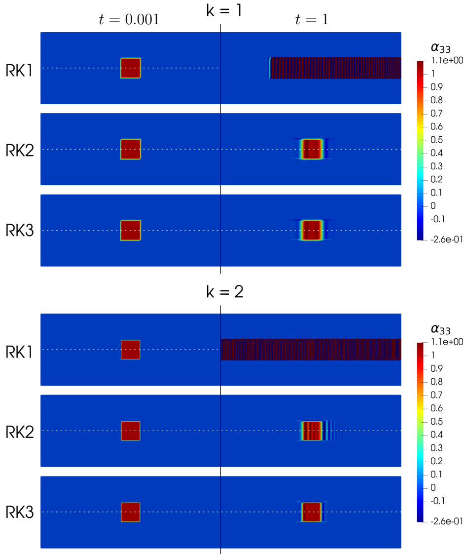
Figure 1: Role of space and time approximations: Comparison between predictions of RK1, RK2 and RK3 schemes for polynomial degree k = 1 and k = 2 (space approximations) for the transport of a single screw dislocation with density \alpha_{33} \text{ nm}^{-1} (initial state defined by (18)) at a constant velocity (19) without slope limiting. The parameters common to all these simulations are \kappa = 1 , no slope limiting, space discretization with (200 \times 40 \times 1) elements, t_F = 1 sec and \delta t = 0.001 sec. The black vertical lines denote the separation between the results after the first time step ( t = 0.001 sec) and the last time step ( t = 1 sec). The dashed lines are the lines along which the line plots in Figure 2 have been generated for the different RK schemes. This plot has been generated in ParaView 5.7.0.
