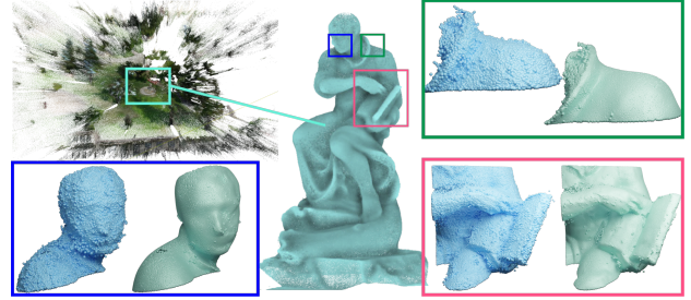
Figure 11: Large-scale denoising II: After applying our method on a large-scale real scanning-scene from [KPZK17] ( \sim 7M points) where noise type and level vary in space, we visualize the original vs. denoised pointset on the statue at the center of the scene in closeup insets: face, collar, hand and book are well reconstructed, with clear sharp features, e.g., on the collar and the open book.
